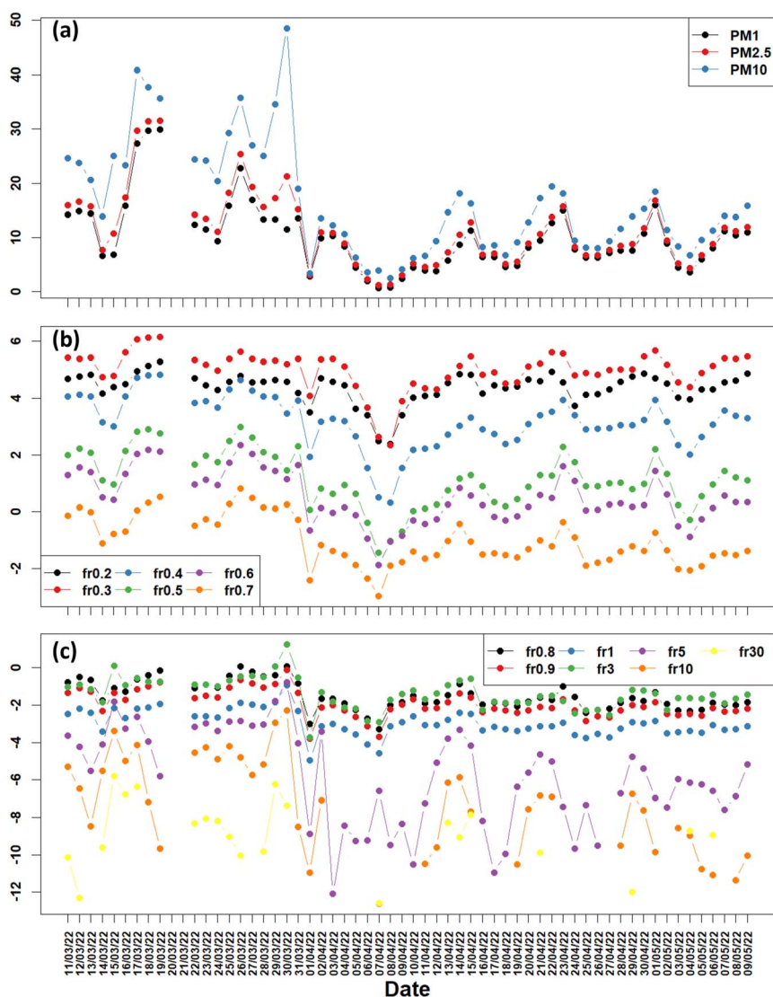
Fig. 3 Time series (daily average) from OPS data of (a) PM 1 , PM 2.5 , and PM 10 (in \mu\text{g m}^{-3} ), (b) fine, and (c) coarse particle fractions (in particles per \text{cm}^3 , logarithmic scale). Discontinuities are due to missing data from the days 20th and 21st March. Reported size fractions correspond to: fr0.2 bin size 0.15–0.2 \mu\text{m} ; fr0.3 0.2–0.3 \mu\text{m} ; fr0.4 0.3–0.4 \mu\text{m} ; fr0.5 0.4–0.5 \mu\text{m} ; fr0.6 0.5–0.6 \mu\text{m} ; fr0.7 0.6–0.7 \mu\text{m} ; fr0.8 0.7–0.8 \mu\text{m} ; fr0.9 0.8–0.9 \mu\text{m} ; fr1 0.9–1.0 \mu\text{m} ; fr3 1.0–3.0 \mu\text{m} ; fr5 3.0–5.0 \mu\text{m} ; fr10 5.0–10.0 \mu\text{m} ; fr30 10.0 \mu\text{m} to the last bin, namely 26.4 \mu\text{m} .
