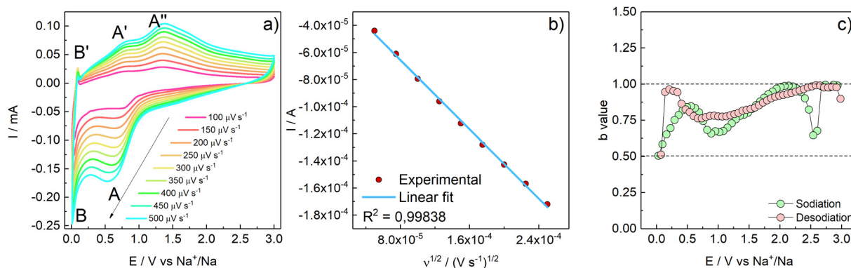
Fig. 6 (a) Cyclic voltammeteries acquired at different scan rates from 100 up to 500 \mu\text{V s}^{-1} (50 \mu\text{V s}^{-1} increment steps). (b) I vs. \nu^{1/2} plot with linear fit of peak A. (c) calculated b -values vs. E .
