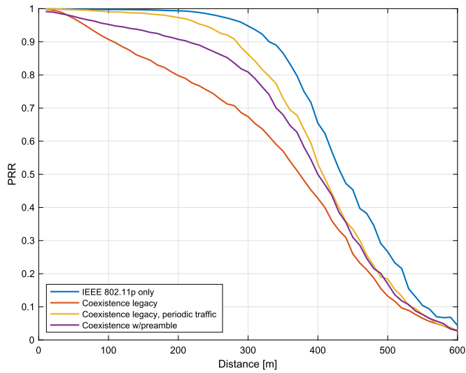
(a) Packet reception ratio of IEEE 802.11p.
