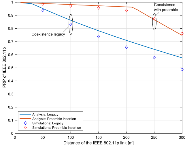
(a) Packet reception probability of the IEEE 802.11p link vs. the link distance, with 1000 LTE-V2X transmissions per kilometer
