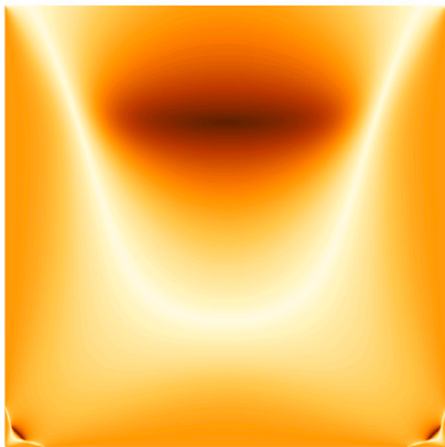
(b) \delta = 0.1
