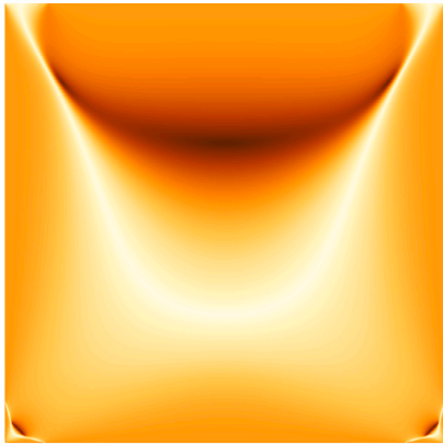
(a) \delta = 0
