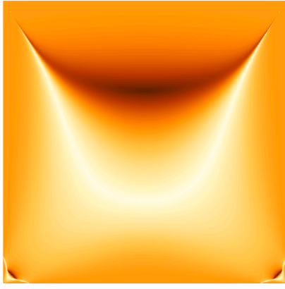
(a) \delta = 0
