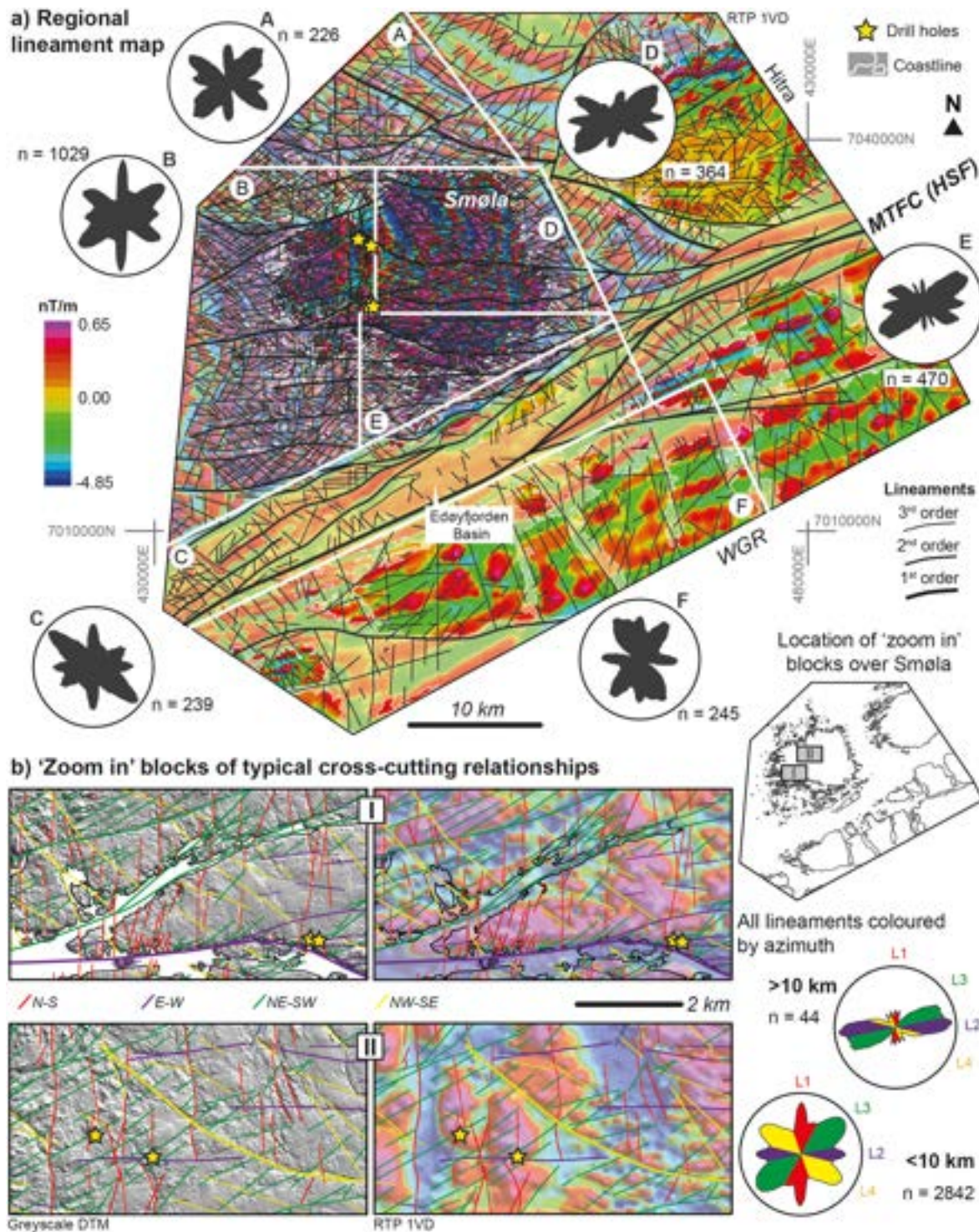
Figure 2. (a) Airborne magnetic survey imagery (reduced to pole-first vertical derivative – RTP-1VD) over Smøla island and surrounding areas (coastline shown in white). Displayed over the magnetic imagery are first-, second-, and third-order lineaments mapped from both the magnetic data and DTM data. Airborne magnetic survey imagery from Nasuti et al. (2015). The area over Smøla onto the WGR region is subdivided into A (north of Smøla), B (west and SW of Smøla), C (area over the MTFC), D (NE Smøla), E (SE Smøla), and F (WGR area). Rose plots of strike trends of mapped lineaments are shown by area. (b) Zoomed-in blocks showing representative examples of crosscutting relationships between the different lineament trends (coloured by trend) on both DTM and geophysical imagery (DTM data from the NGU). Locations of the zoomed-in blocks are displayed on the adjacent schematic map of Smøla (coastline map courtesy of the NGU), along with rose diagrams showing orientation trends of lineaments with > 10 and < 10 km lengths. Rose plots use the same colours as the lineaments on the zoomed-in blocks and are labelled to show the L1 to L4 lineament trends.
