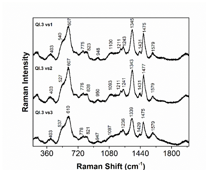
Figure S1. Raman spectra for the ink various versions of QI.3, applied on filter paper, \lambda = 750\text{nm}
