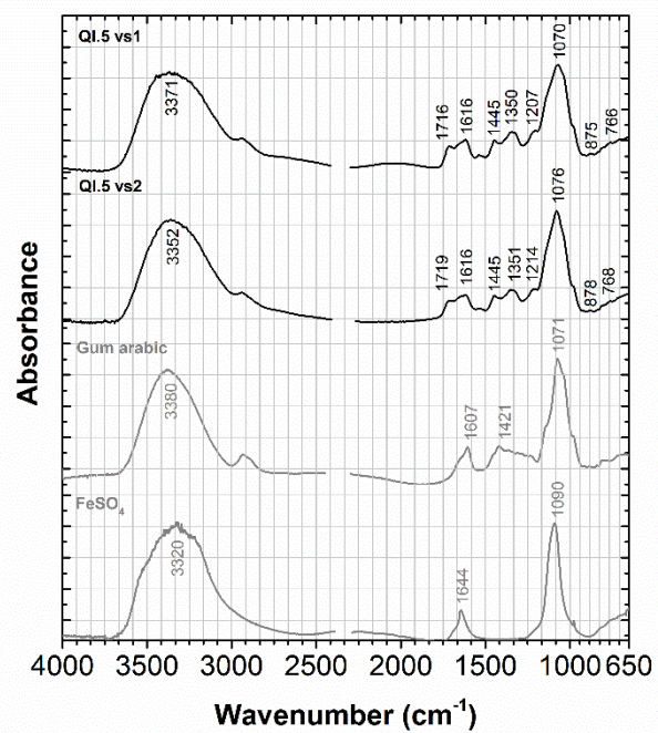
Figure S6. IR spectra for the ink various versions of QI.5.
