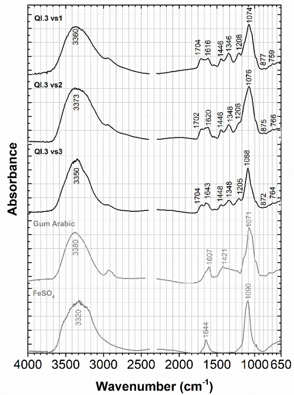
Figure S4. IR spectra for the ink various versions of QI.3.
