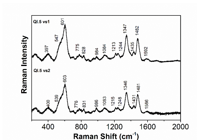
Figure S3. Raman spectra for the ink various versions of QI.5, applied on filter paper, \lambda = 750\text{nm}
