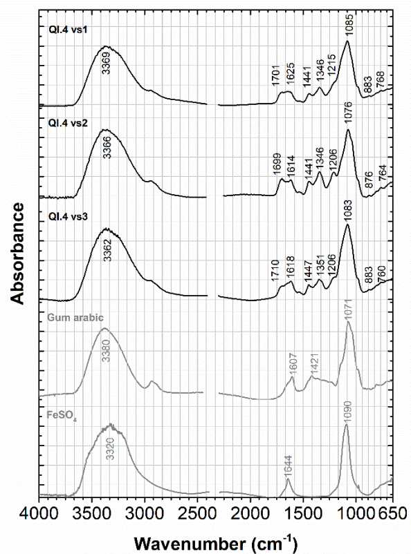
Figure S5. IR spectra for the ink various versions of QI.4.
