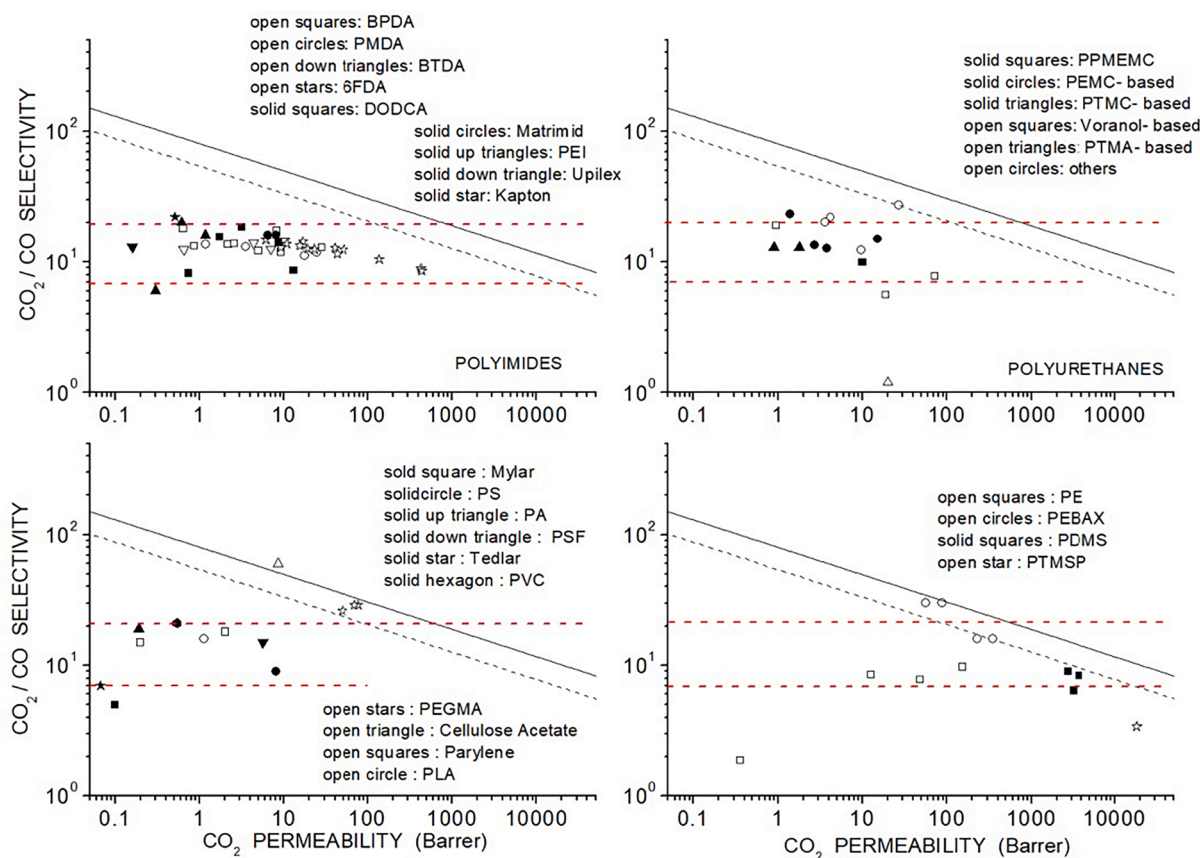
Fig. 4. CO_2/CO ideal selectivity ( \alpha ) of the discussed polymeric films. (upper left). Polyimides [72–76,80,81,83,85]. (upper right). Polyurethanes [104,104]. (lower left). Green polymers [80,82,96,98,100], PEGMA-co-MMA-co-BPMA [76], Polyester, Mylar [82,113], polystyrene [82,110], PSF [61, 97, 98 82,118,119], PVF [82,107], PVC [65–69]. (lower right). polyethylene [62] and High Free Volume polymers [76,92,93]. The solid lines in all figures mark the upper bound defined by eq. (13) while the dotted lines are the upper bound as reported in [80]. The dashed horizontal lines mark the \alpha = 7 and \alpha = 20 values. (For interpretation of the references to color in this figure legend, the reader is referred to the web version of this article.)
