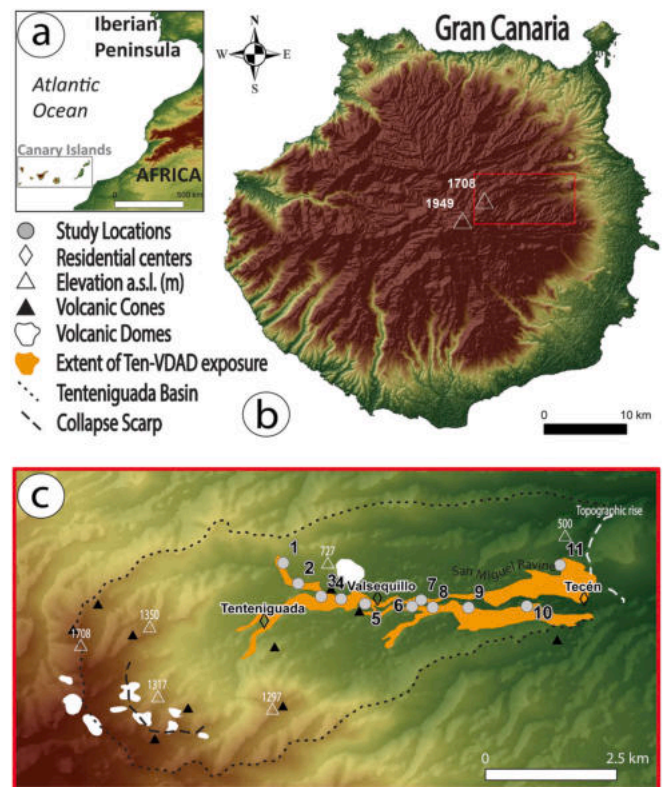
Fig. 1. a Location of the Canary Islands. b The Island of Gran Canaria with the location of the Tenteniguada basin (red rectangle – also indicates the extent of c). c The Tenteniguada debris avalanche deposit is exposed on the walls of the San Miguel Ravine in the Tenteniguada basin due to fluvial incision. (For interpretation of the references to colour in this figure legend, the reader is referred to the web version of this article.)
