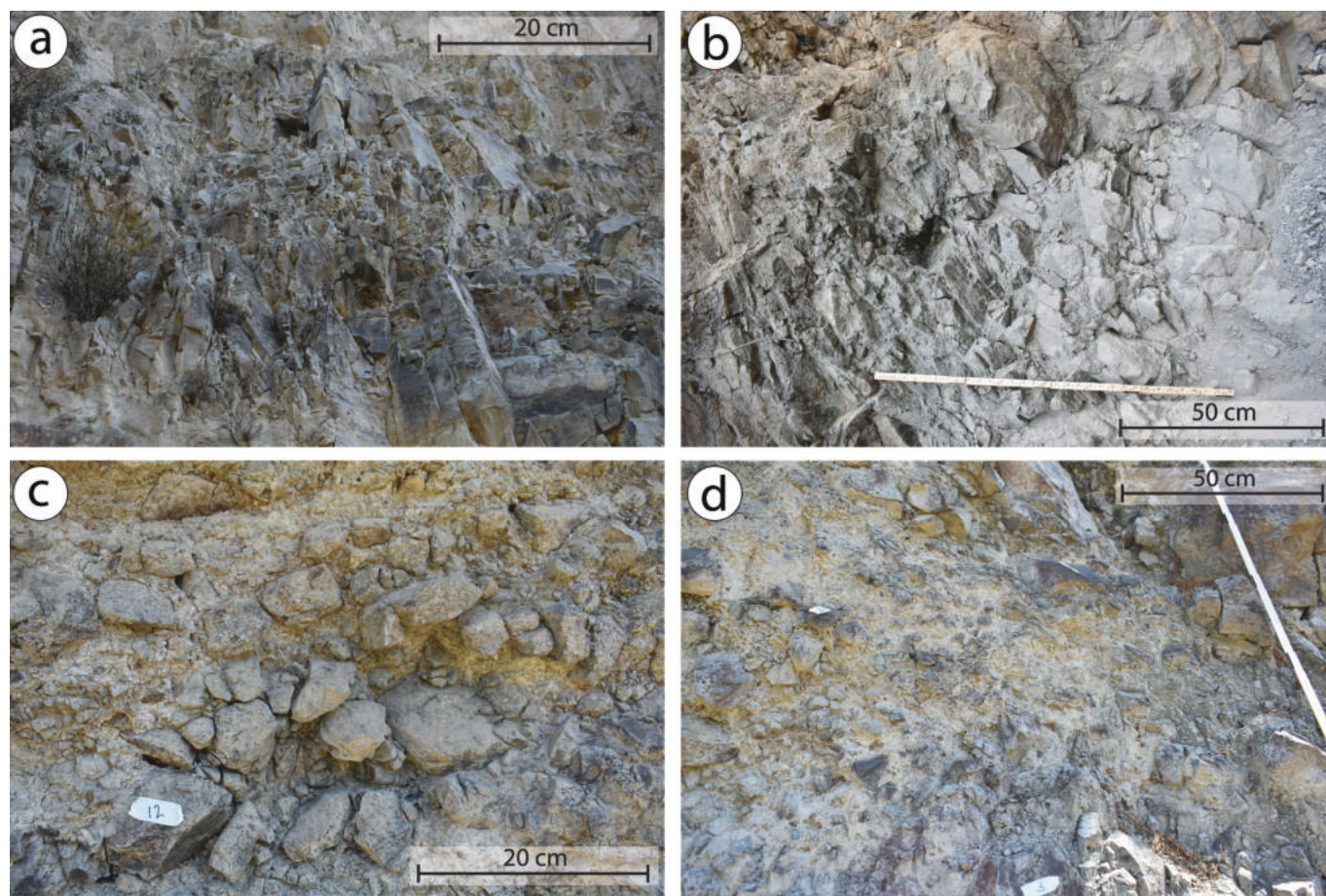
Fig. 7. Stages of disaggregation from jigsaw-fractured block to monolithological diamicton illustrated through blocks at different stages of disaggregation. a Undisaggregated jigsaw-fractured block where the components are not displaced (location 2). b In this block angular clasts composing the jigsaw-fit fabric preserve their original order, however, small quantity of fine material has been generated between them (location 9). c The original structure of the component clasts has been eliminated and the block has the fabric of a monolithologic breccia (location 10). d The block here exhibits the texture of a matrix enriched, disaggregated, matrix-supported monolithological diamicton (location 2).
