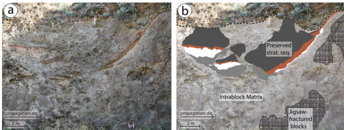
Fig. 4. The outcrop in location 4 is composed of a block with components of variable disaggregation. It exhibits a component of preserved stratigraphy higher up in the outcrop, and jigsaw-fractured undisaggregated components lower down. The rest of the block is composed of an intrablock matrix. a Red horizons illustrate stratigraphic preservation (red shaded area in b). Person for scale. b Annotated image of the same outcrop. The dashed line marks the top of the deposit. The shaded areas represent distinct lithological units, illustrating the preserved stratigraphy. (For interpretation of the references to colour in this figure legend, the reader is referred to the web version of this article.)
