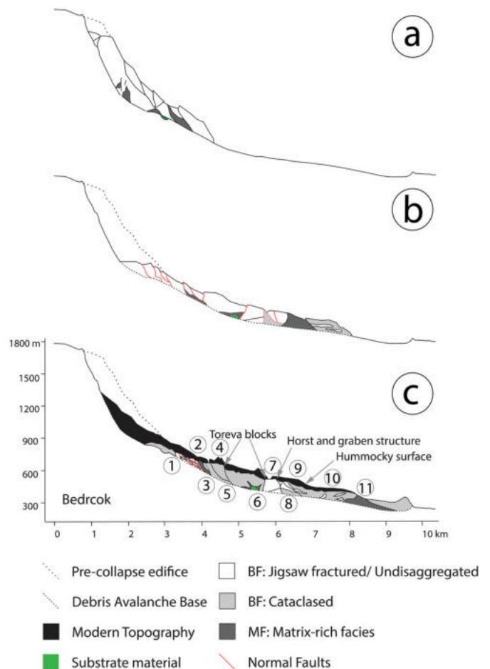
Fig. 13. Schematic representation of the propagation and emplacement of the Teneniguada debris avalanche. a The initial stage of the collapse and coarse fracturing of the material. b Propagation stage where fractures are activated as normal faults to accommodate the spreading of the mass. c The final deposit with the features that have been observed in the field. Circled number represent the study locations as listed illustrated on the map in Fig. 1 and the table in the complementary material Appendix A.
