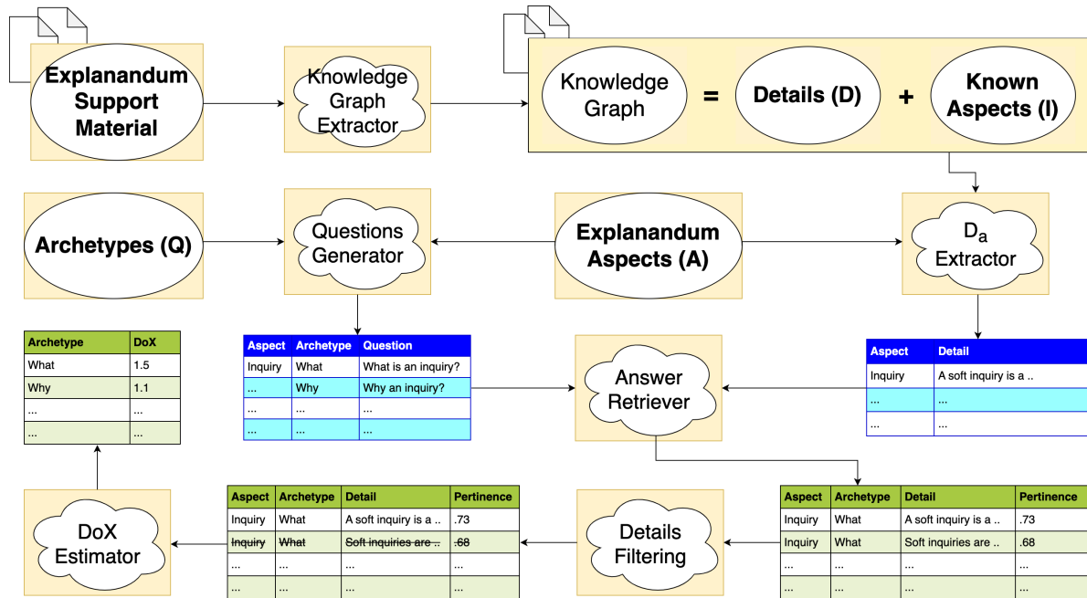
Figure 2: DoXpy Pipeline. The pipeline starts with extracting a graph from the explanandum support material \Phi that is then converted into a set of details D . The set of details is then used with the explanandum A and the set of archetypes Q to compute the DoX. To do this, we use some deep language models for answer retrieval.
