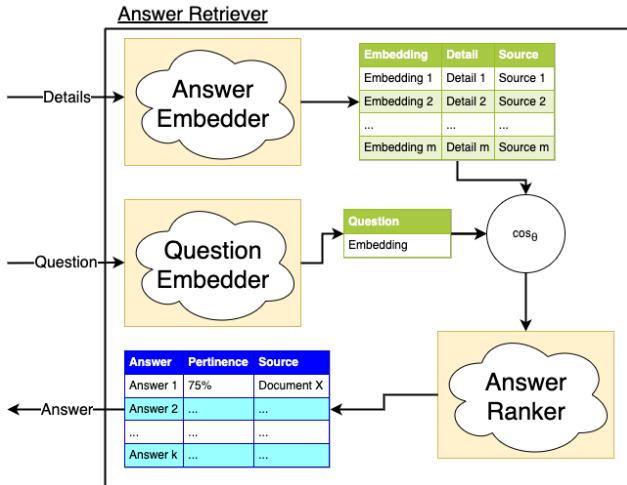
Figure 1: Flow Diagram of the Answer Retriever used in the pipeline of DoXpy. This figure summarises the answer retrieval algorithm used by DoXpy. A question q_a is given as input to the retriever together with a set of details D_a . Then, the details in D_a and q_a are embedded, and their cosine similarity ( \theta ) is used to rank details according to their pertinence to the question.
