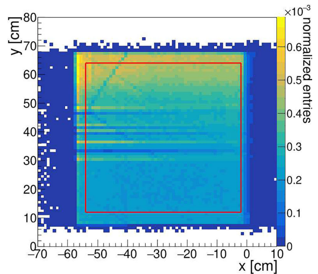
Fig. 8 Distribution of DS tracks at the most upstream detector plane. The distribution is normalized to unit integral. Horizontal stripes in the central part of the detector are caused by scintillator bar inefficiencies. The red border delimits the region considered for the DS muon flux measurement
