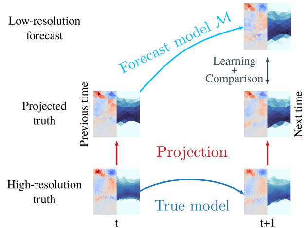
Figure 3. In our twin experiments, the high-resolution state with a 4 km resolution is propagated from time t to time t + 1 with the high-resolution true model; one discrete time step corresponds here to a lead time of 10 min and 8 s. The high-resolution truth at time t is projected by Lagrange interpolation into low-resolution space (8 km resolution), acting as initial state for the forecast. The forecast is performed by the low-resolution forecast model \mathcal{M} , which propagates the state from time t to time t + 1 in the low-resolution space. The model error correction is learned by comparing the low-resolution forecast at time t + 1 to the truth at the same time, projected into low-resolution space.
