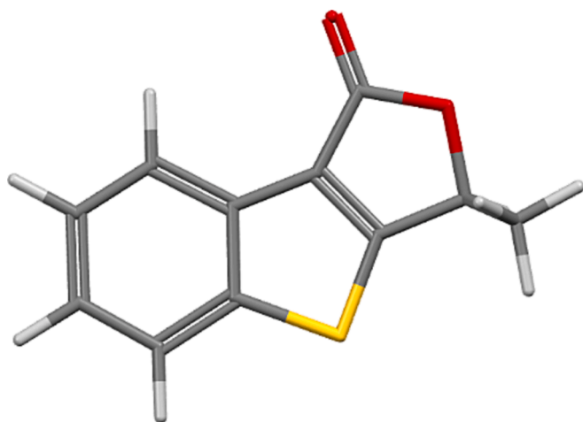
Fig. 1. X-ray molecular structure of 3-methylbenzo[4,5]thieno[2,3-c]furan-1-one 2a .
