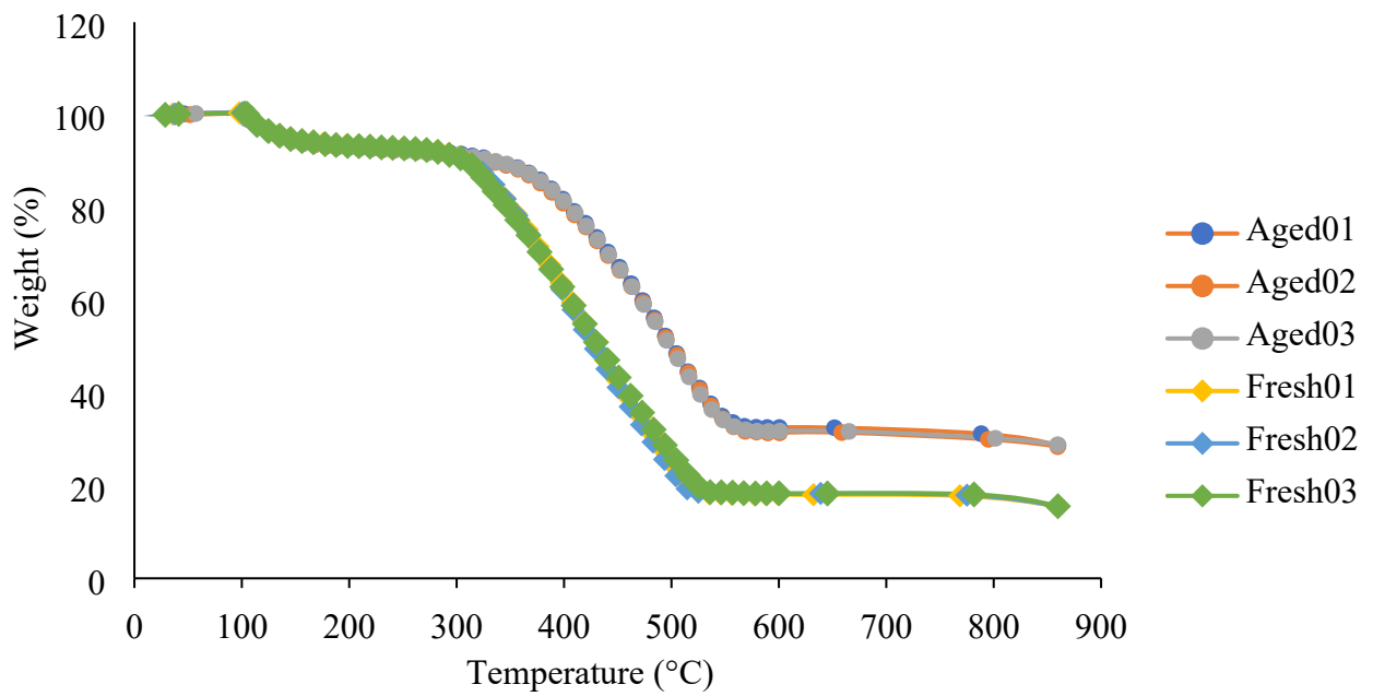
Figure SM2. Thermogravimetric (TG) curves obtained from fresh and aged biochar applied in the field experimental.
