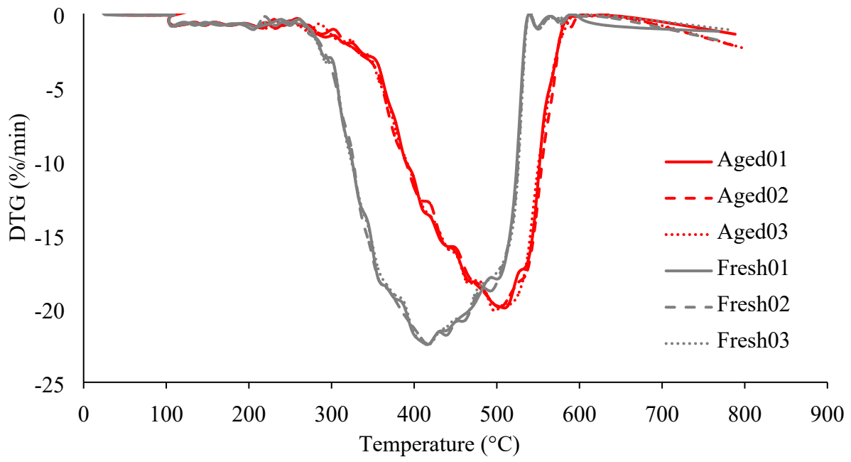
Figure SM3. Derivative thermogravimetric (DTG) curves obtained from fresh and aged biochar applied in the field experimental.
