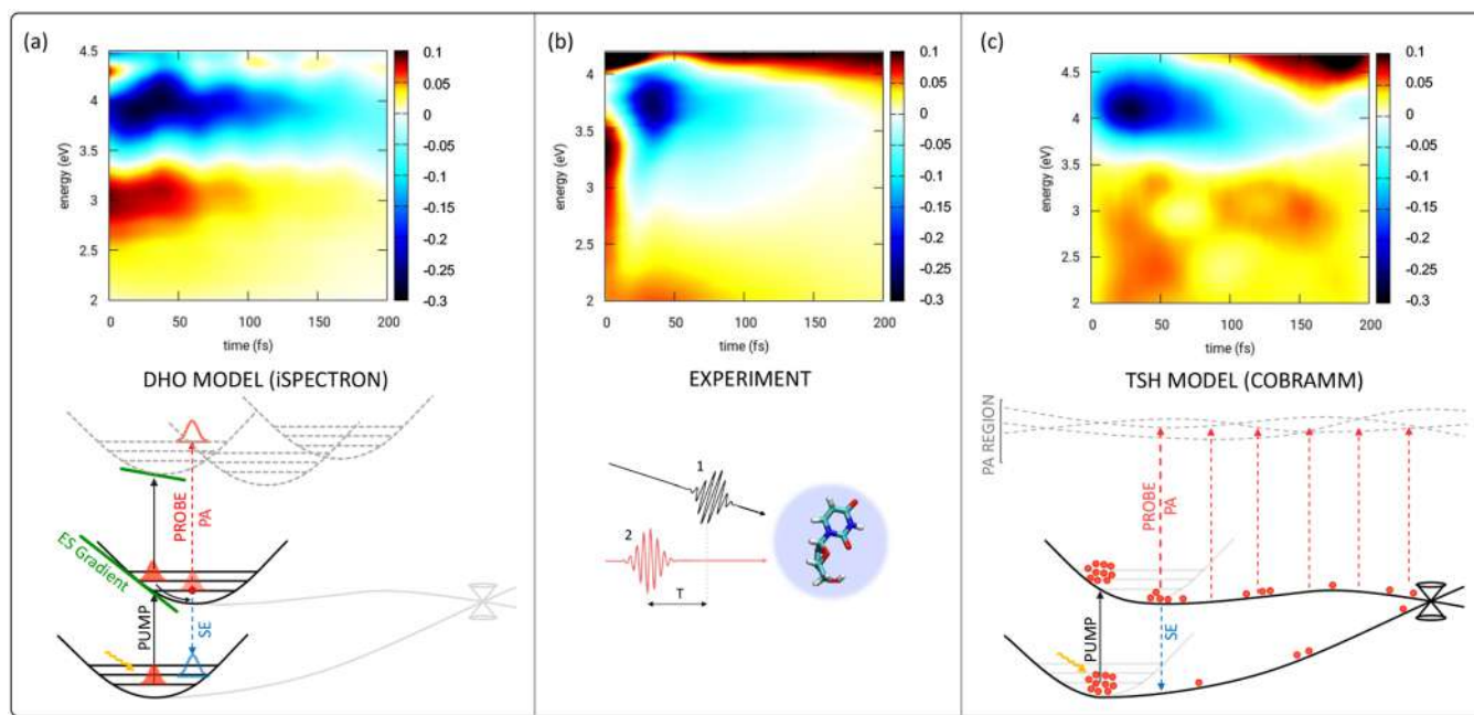
Figure 29. Spectra and schemes for simulated (a,c) and recorded (b) UV/vis transient absorption spectroscopy of water solvated Uridine. (a) Spectrum (top) based on the DHO model (bottom), obtained with the OpenMolcas/Spectron interface iSpectron; (b) Experimental map (top) and schematic representation of the experimental setup (bottom); (c) Spectrum (top) based on TSH model (bottom), obtained via the OpenMolcas/COBRAMM interface.
