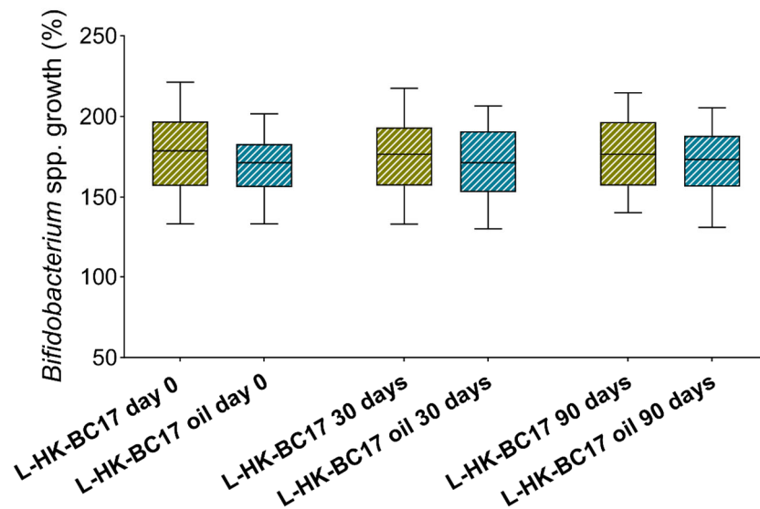
Figure 8. Effects of L-HK-BC17 and L-HK-BC17 oil on planktonic cultures of Bifidobacterium spp. over time. The effects of L-HK-BC17 and L-HK-BC17 oil were tested at 10^7 heat-killed cells/mL immediately after preparation (day 0) and after 30 days and 90 days of storage. Each box represents the interquartile range (25th and 75th percentiles), and lines within the boxes indicate the median values for the samples. The extremes of the bars indicate the minimum and maximum values, respectively.
