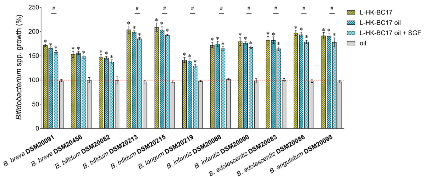
Figure 5. Bifidogenic activity of formulated HK-BC17. The effects of sunflower oil, L-HK-BC17, L-HK-BC17 oil (the not-digested and digested in simulated gastric fluid (SGF)) ( 10^7 heat-killed cells/mL) on planktonic cultures of Bifidobacterium spp. are expressed as percentages with respect to the control (100%, red line) (mean \pm SD, n = 3 ). *, p < 0.05 . Statistical differences between the not-digested and digested L-HK-oil are also shown; #, p < 0.05 .
