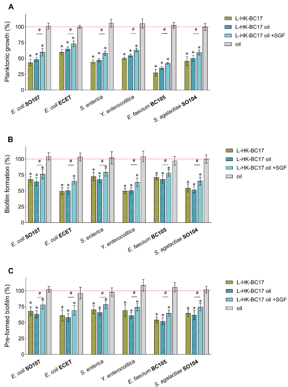
Figure 7. Effects of formulated HK-BC17 on human pathogens. Effects of sunflower oil, L-HK-BC17, L-HK-BC17 oil (the not-digested and digested in simulated gastric fluid (SGF)) ( 10^7 heat-killed cells/mL) on planktonic cultures (A), biofilms formation (B), and pre-formed biofilms (C) of E. coli SO107, enterotoxigenic E. coli (ETEC), S. enterica , Y. enterocolitica , E. faecium BC105, and S. agalactiae SO104. Biofilms were quantified by CV staining. Results are expressed as percentages with respect to the control (100%, red line, mean \pm SD, n = 3 ); *, p < 0.05 Statistical differences between the not-digested and digested L-HK-BC17 oil are also shown; #, p < 0.05 .
