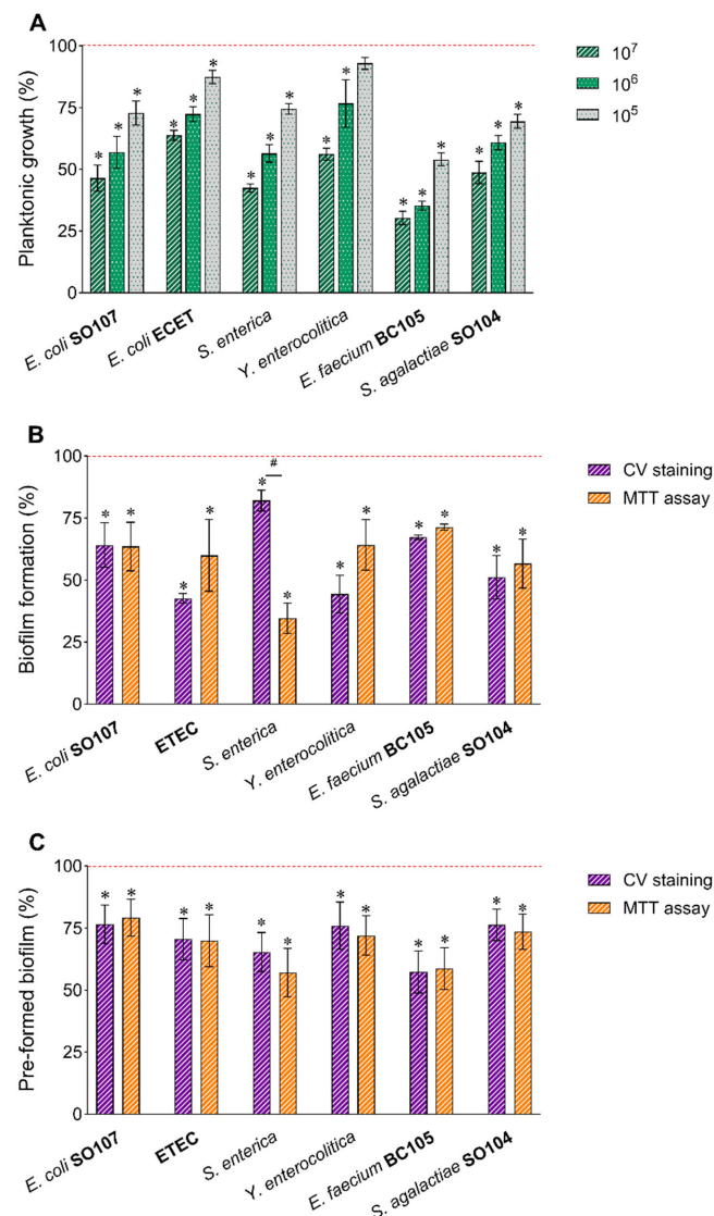
Figure 3. Effects of HK-BC17 on human pathogens. Effects of HK-BC17 at three concentrations ( 10^7 , 10^6 and 10^5 heat-killed cells/mL) on planktonic cultures of E. coli SO107, enterotoxigenic E. coli (ETEC), S. enterica , Y. enterocolitica , E. faecium BC105 and S. agalactiae SO104 (A). Effects of HK-BC17 ( 10^7 heat-killed cells/mL) on biofilms formation (B) and pre-formed biofilms (C) of the same pathogens quantified by CV staining and MTT assay. Results are expressed as percentages with respect to the control (100%, red line, mean \pm SD, n = 3 ); *, p < 0.05 . Statistical differences between CV and MTT methods are also shown; #, p < 0.05 .
