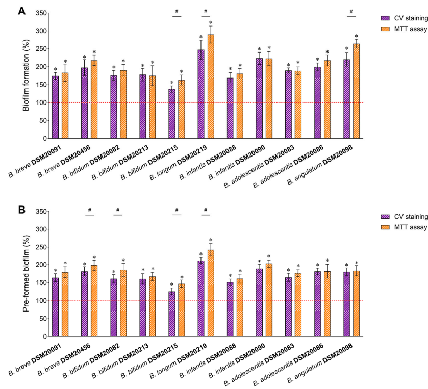
Figure 2. Effects of HK-BC17 ( 10^7 heat-killed cells/mL) on biofilms formation (A) and pre-formed biofilms (B) of Bifidobacterium spp. Biofilms are quantified by CV staining and MTT assay. Results are expressed as percentages with respect to the control (100%, red line) (mean \pm SD, n = 3 ); *, p < 0.05 . Statistical differences between the two methods are also shown; #, p < 0.05 .
