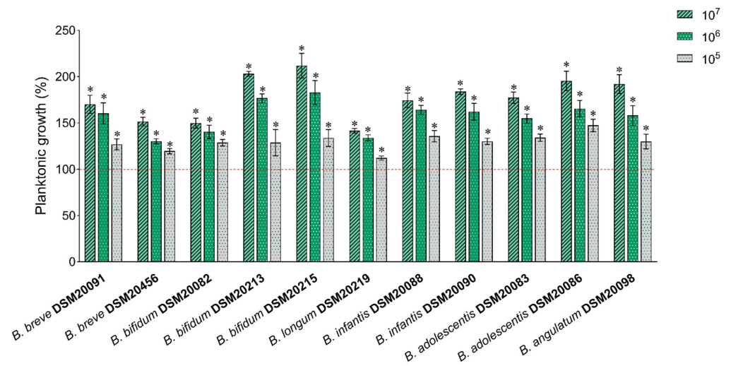
Figure 1. Bifidogenic activity of HK-BC17. The effects of HK-BC17 at three concentrations ( 10^7 , 10^6 and 10^5 heat-killed cells/mL) on planktonic cultures of Bifidobacterium spp. are expressed as percentages with respect to the control (100%, red line) (mean \pm SD, n = 3 ); *, p < 0.05 .
