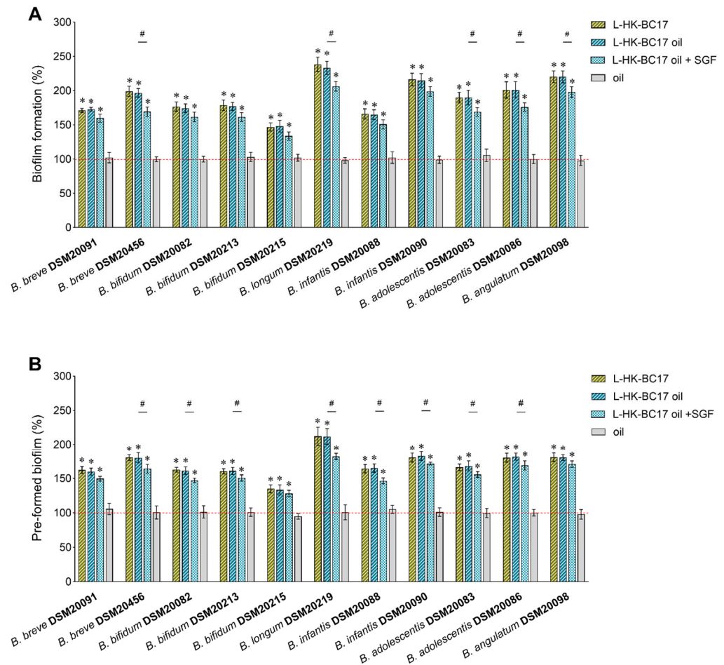
Figure 6. Biofilm-stimulating activity of formulated HK-BC17. The effects of sunflower oil, L-HK-BC17, L-HK-BC17 oil (the not-digested and digested in simulated gastric fluid (SGF)) ( 10^7 heat-killed cells/mL) on biofilms formation (A) and pre-formed biofilms (B) of Bifidobacterium spp. are quantified by CV staining and expressed as percentages with respect to the control (100%, red line) (mean \pm SD, n = 3 ). *, p < 0.05 . Statistical differences between the not-digested and digested L-HK-BC17 oil are also shown; #, p < 0.05 .
