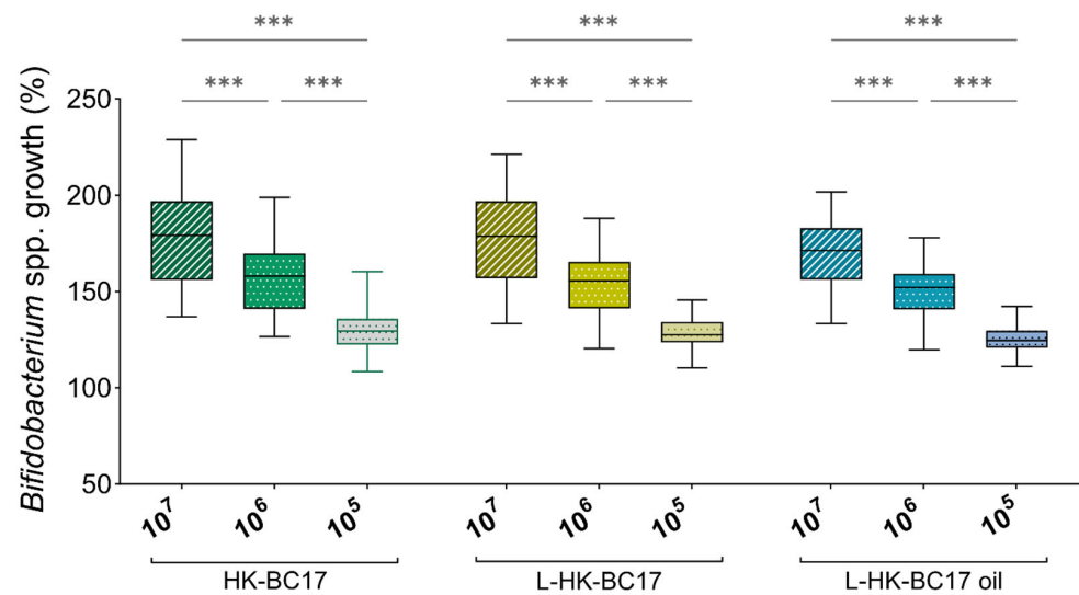
Figure 4. Effects of HK-BC17, L-HK-BC17 and L-HK-BC17 oil on planktonic cultures of Bifidobacterium spp. HK-BC17, L-HK-BC17 and L-HK-BC17 oil were tested at three concentrations ( 10^7 , 10^6 and 10^5 heat-killed cells/mL). Each box represents the interquartile range (25th and 75th percentiles), lines within the boxes indicate the median values for the samples. The extremes of the bars indicate the minimum and maximum values, respectively.***, p < 0.001 .
