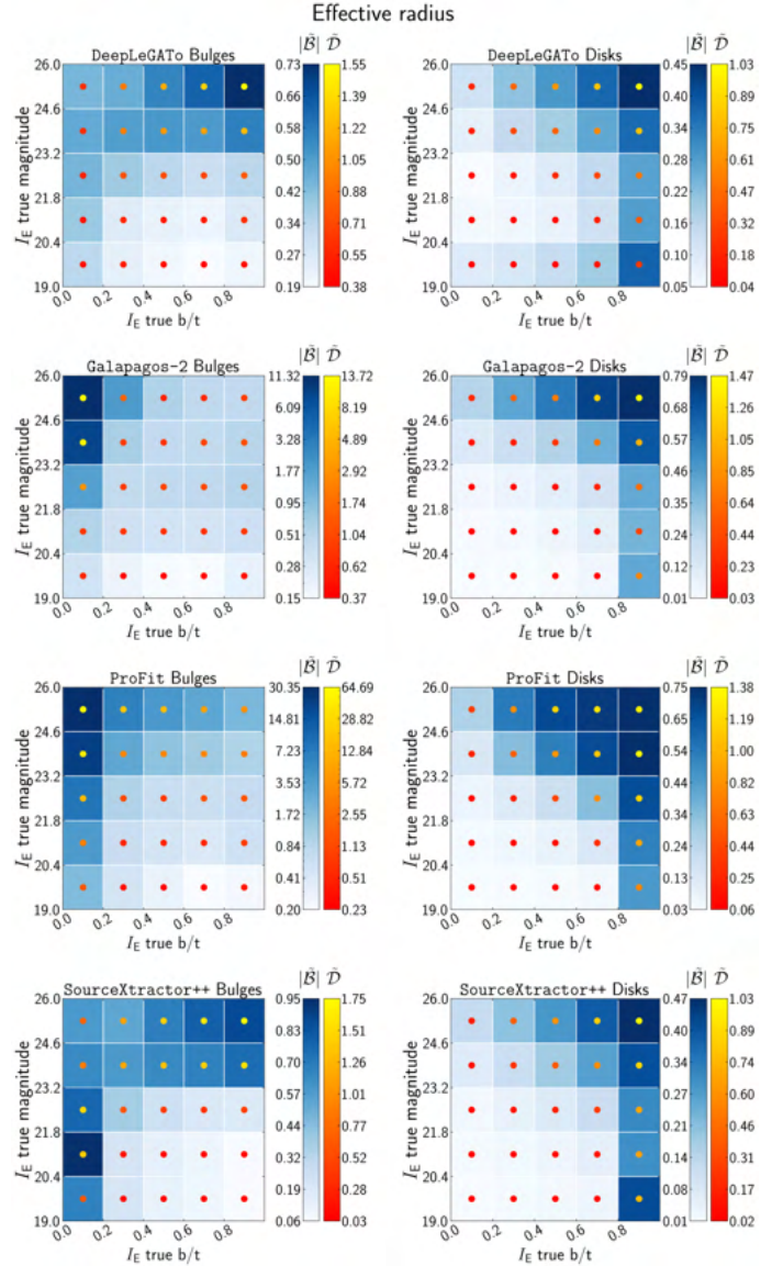
Fig. 9. Absolute bias |\bar{B}| and dispersion \bar{D} for the effective radius of bulge (left column) and disc (right column) components in the double-Sérsic simulation, as a function of bulge-to-total ratio ( x -axis) and apparent I_E magnitude ( y -axis). Each row shows a different code. For ProFit and Galapagos-2, the colour scale is logarithmic. In each panel, the colour of the squares is proportional to the mean bias \mathcal{D} (lighter being smaller), and the colour of the dot inside each square indicates the dispersion \mathcal{D} (redder being lower). For most of the codes, we find the expected behaviour: both the bias and the dispersion increase for faint objects, as well as at small b/t for bulges and large b/t for discs.
