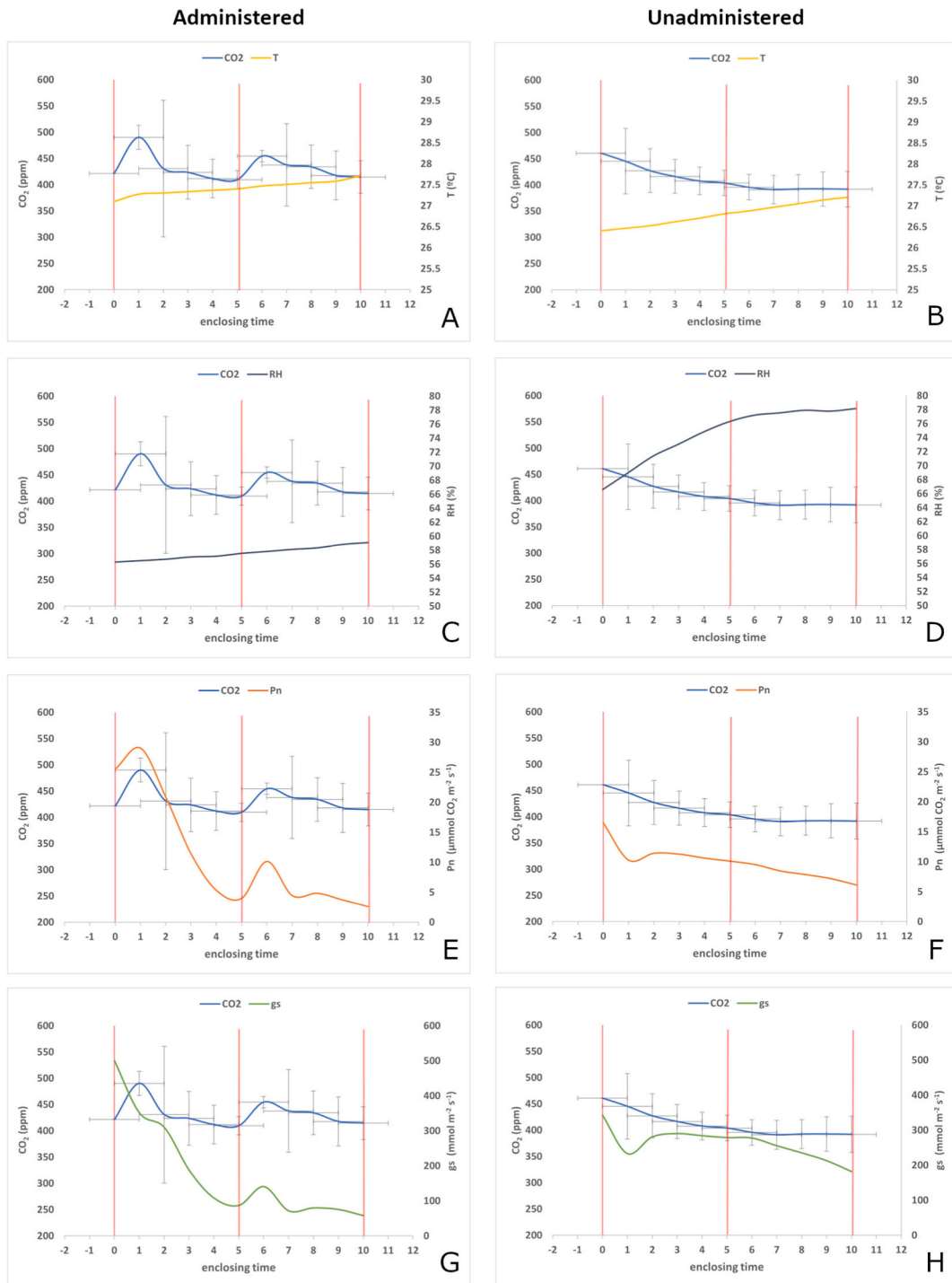
Fig. 4. Mean \pm SD of \text{CO}_2 levels interpolated with the monitored environmental variables (T: 'A' and 'B'; RH: 'C' and 'D') and predicted physiological ones (Pn: 'E' and 'F'; gs: 'G' and 'H') under administered (left) and unadministered (right) \text{CO}_2 condition along plant enclosure sampling. Red bars delimit the principal sampling intervals considered (5- and 10- minutes).
