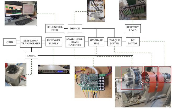
Fig. 16. Test bench.
