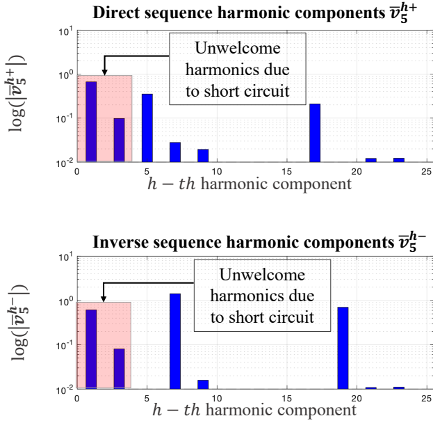
Fig. 6. Time-harmonic contributions to the space vector \bar{v}_5 . The significant terms that appear in \bar{v}_{5,DS} due to a short circuit fault are highlighted.
