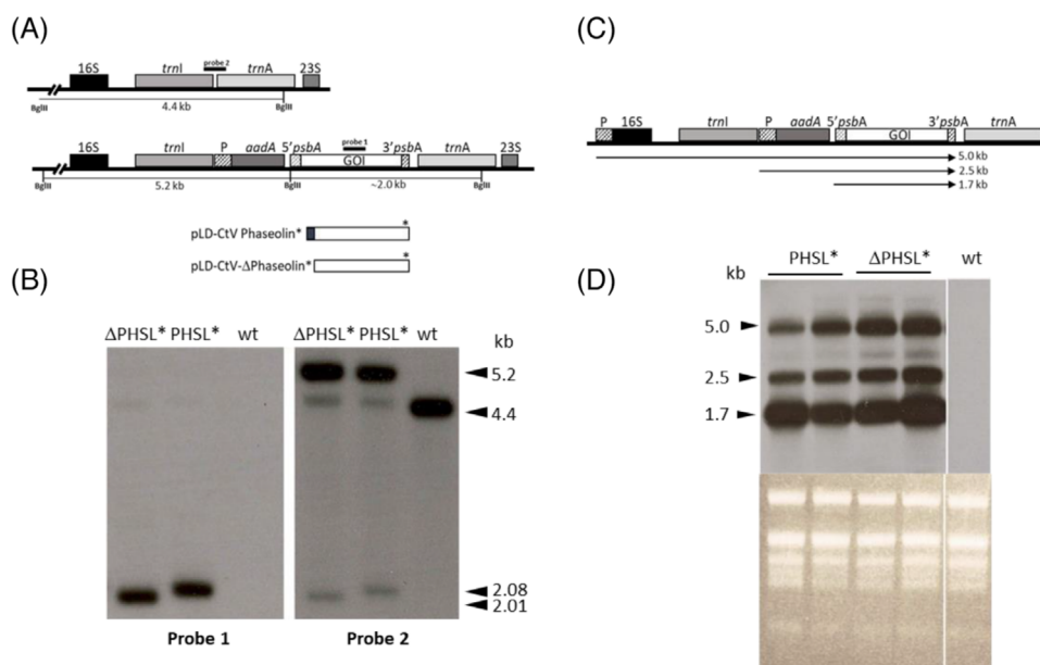
FIGURE 1 Northern and Southern blot analyses of tobacco transplastomic plants. (A) Schematic representation of the 16S/trnI/trnA/23S region of the tobacco chloroplast genome and of the plastid transformation vectors, the probes used for Southern blot analysis are indicated as probe1 ( phaseolin gene) and probe2 ( trnI/trnA region). The predicted hybridizing fragments, after digestion with BglIII restriction enzyme and Southern blot analysis, are indicated in kb. (B) Southern blot analysis of PHSL* and ΔPHSL* transformants with probe1, phaseolin gene (left panel), and probe 2, trnI/trnA region (right panel), showing transgenes plastome integration. The probe 1 produced two slightly different fragments due to the absence of the DNA sequence coding for the signal peptide in the ΔPHSL* plant. The faint fragments around 4.5 kb in the transplastomic plants are likely promiscuous plastid DNA already present in the nucleus, as already reported. [13] (C) Scheme of the transcription pattern expected for the transplastomic PHSL* and ΔPHSL* genes (GOI). Horizontal arrows represent expected transcripts and their sizes. (D) Northern blot analysis on total RNA extracted from PHSL*, ΔPHSL*, and wild type (wt) plants. As a loading control, rRNA stained by ethidium bromide is shown in the lower panel. The wt sample is shown separately but belongs to the same agarose gel, which contained other four RNA samples close to the wt lane that have been not shown because not inherent to this study. Phaseolin gene was used as a probe. Numbers indicate molecular mass markers in kb. P, Prn promoter; aadA, aminoglycoside 3'-adenylyl transferase gene; 5'psbA, psbA promoter/5'UTR; 3'psbA, psbA terminator; GOI, gene of interest.
