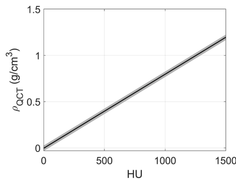
Fig. 6. The calibration line employed to derive density from the CT Hounsfield Units. The shaded area highlights the uncertainty associated to the average over a varying number of HU.
