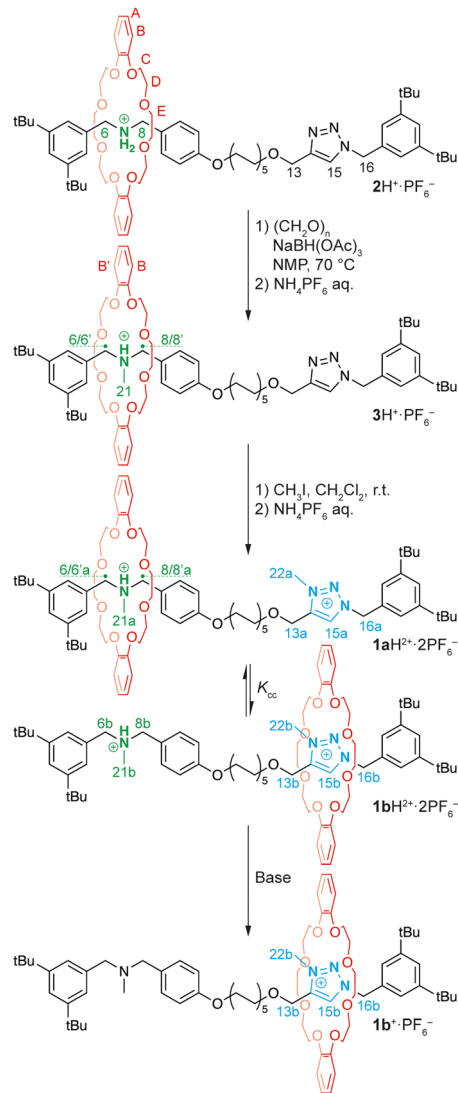
Scheme 1 Synthesis and coconformational equilibrium of rotaxane 1aH 2+ ·2PF 6 - and 1bH 2+ ·2PF 6 - .
