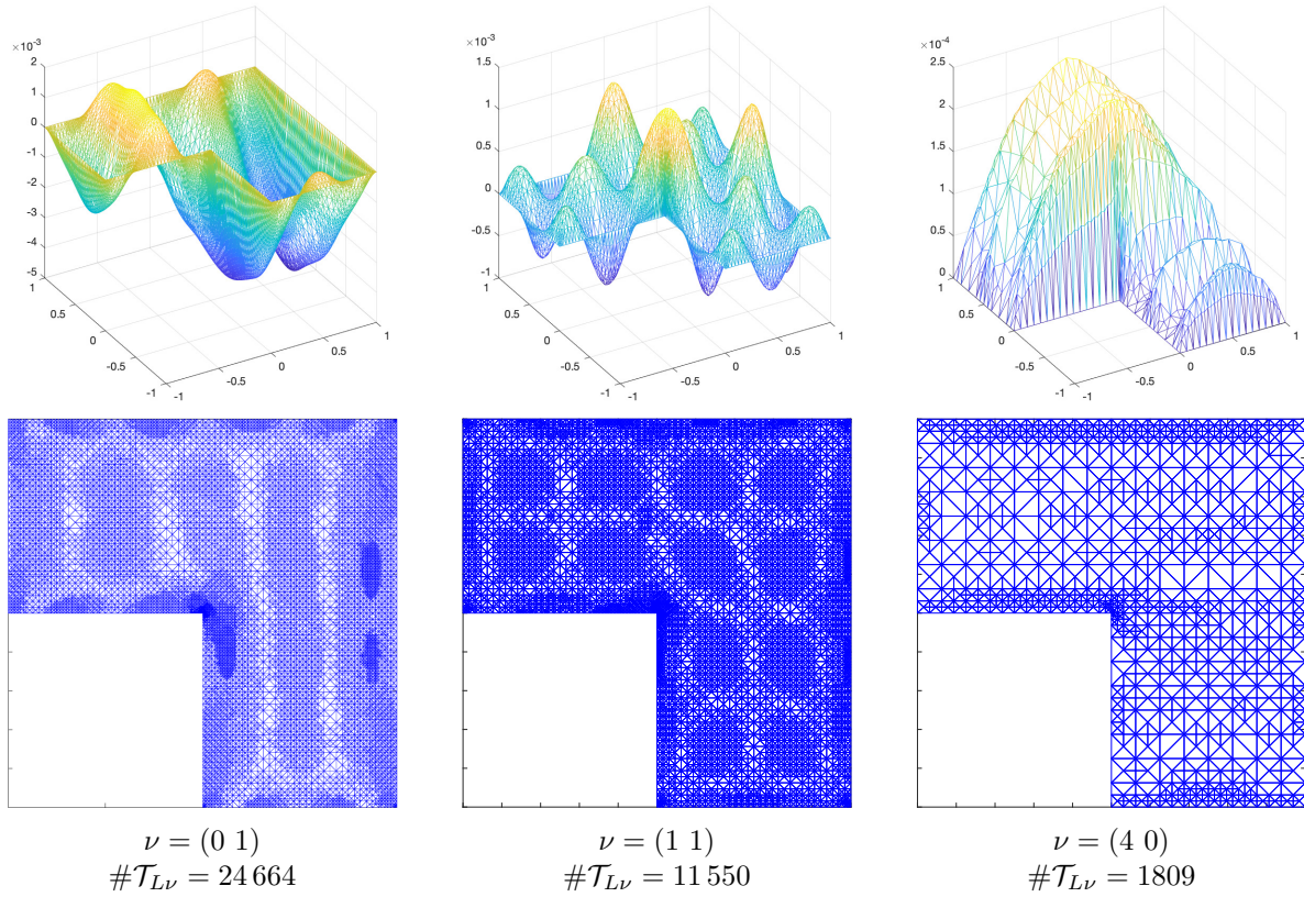
Figure 4: Experiments in subsection 7.1.2 : Coefficients u_{L\nu} \in \mathbb{X}_{L\nu} = \mathcal{S}^1(\mathcal{T}_{L\nu}) of the final SGFEM approximation generated by ML-C (top plots) and the associated adaptively refined meshes \mathcal{T}_{L\nu} (bottom plots) for three indices \nu \in \mathfrak{P}_L .
