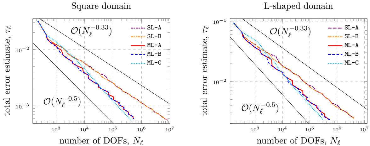
Figure 2: Experiments in subsection 7.1.1 (left) and subsection 7.1.2 (right): Total error estimates \tau_\ell versus the number of degrees of freedom N_\ell for all adaptive algorithms.
