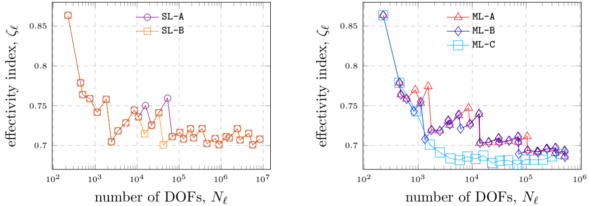
Figure 1: Experiments in subsection 7.1.1 : Effectivity indices \zeta_\ell for the error estimates \tau_\ell in the SGFEM approximations generated by single-level (left) and multilevel (right) adaptive algorithms.
