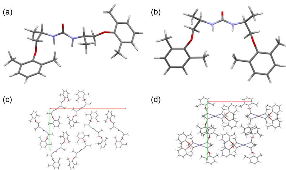
FIGURE 2 Crystal structures of (S,S)-8 (a, c) and (R,S)-8 (b, d). (a, b) Asymmetric unit with color legend: carbon (light gray), hydrogen (white), oxygen (red), nitrogen (blue). (c, d) Packing in the crystal cell, where all hydrogen atoms have been removed for clarity. The unit cell of both molecules is shown in perspective view along the c -axis.
