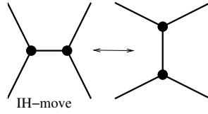
FIGURE 2.3. The IH-move.
