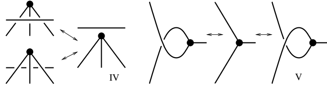
FIGURE 2.2. Reidemeister moves IV and V involve a trivalent vertex.
