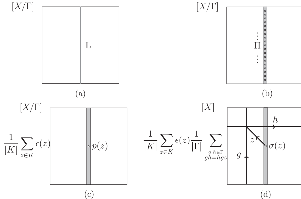
Figure 1. We illustrate the computation of a T^2 correlation function in the orbifold theory [X/\Gamma] with one-cycle L wrapped by a condensation defect, as shown in (a). In (b)–(d) the cycle is shaded gray for visualization purposes, but the only insertions along the cycle are the point operators shown. The prescription is to insert a projection point operator \Pi at every vertex point in some sufficiently fine triangulation of L , as in (b). Since L is connected, it is sufficient to insert \Pi at a single point, and we can write \Pi as a sum over twist fields p(z) , shown in (c). Finally, to compute these correlation functions in terms of the parent theory [X] , we lift each diagram and sum over all consistent ways of inserting \Gamma lines. In the lift, the p(z) operator becomes an operator \sigma(z) sitting on the end of a z line. We can choose where that line joins the other lines. One choice (where they all meet at a junction of degree five) is shown in (d) and it is implicit in our lift that the product of lines around the junction should be the identity, giving the requirement gh = hg .
