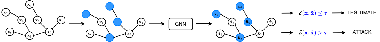
Figure 5: The UAD workflow. The NDN network is converted into an equivalent graph. Randomly selected nodes are masked (blue vertices), and the GNN model aims at reconstructing their feature vectors. An attack is detected when the error score \mathcal{E} between reconstructed and original vectors of masked nodes overcomes threshold \tau .
