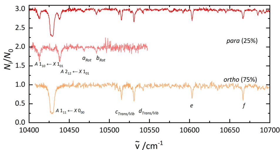
Figure 4. Electronic spectra of \text{H}_2\text{O}@C_{60}^+ (top), p\text{-H}_2\text{O}@C_{60}^+ (middle), and o\text{-H}_2\text{O}@C_{60}^+ (bottom). The lower two traces were obtained in 2 colour experiments. The middle spectrum was recorded by fragmenting all complexes that absorb at 10,429\text{ cm}^{-1} . The bottom spectrum was recorded after irradiation at 10,438\text{ cm}^{-1} .
