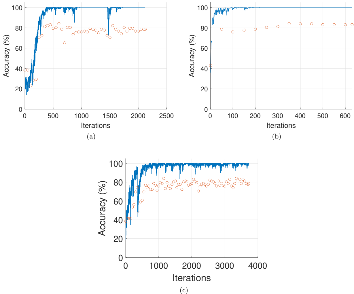
Figure 2. Accuracy plot of GoogLeNet (a), ResNet (b) and AlexNet (c) respect to the training iterations. Training Accuracy (-) and Validation Accuracy ( \circ )
