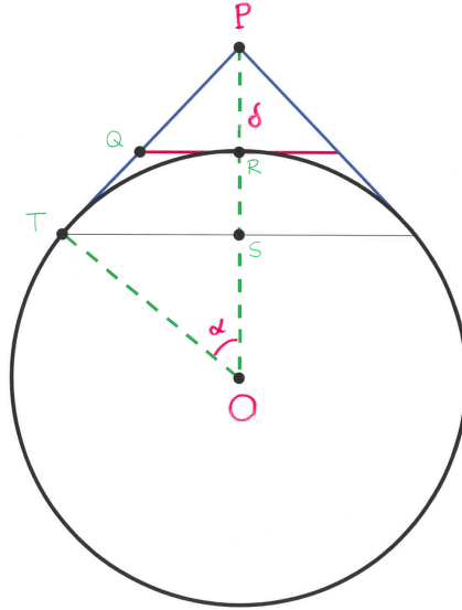
FIGURE 2. The convex hull of B_1 \cup P .
