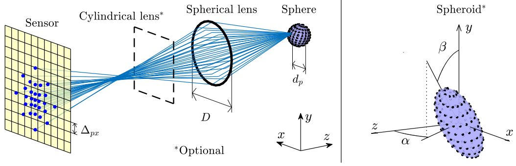
FIG. 2. General concept of MicroSIG. Tracer particles are spheres or spheroids, with light point-sources uniformly distributed on the surface. The path of each ray going through a spherical lens (and optionally also a cylindrical lens) is calculated. The intensity of one pixel is calculated as the count of rays hitting its area. A sketch of a spheroid particle with e_p = 3 and its respective orientation angles \alpha and \beta is presented on the right panel.
