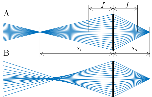
FIG. 1. (A) Ray tracing using a perfect thin lens: Rays originated from a point source at distance s_o from the lens converge to a single point at distance s_i , following the formula 1/s_i + 1/s_o = 1/f , being f the focal lens of the lens. (B) Ray tracing using a spherical lens: Rays originated from a point source do not converge to a single point.
