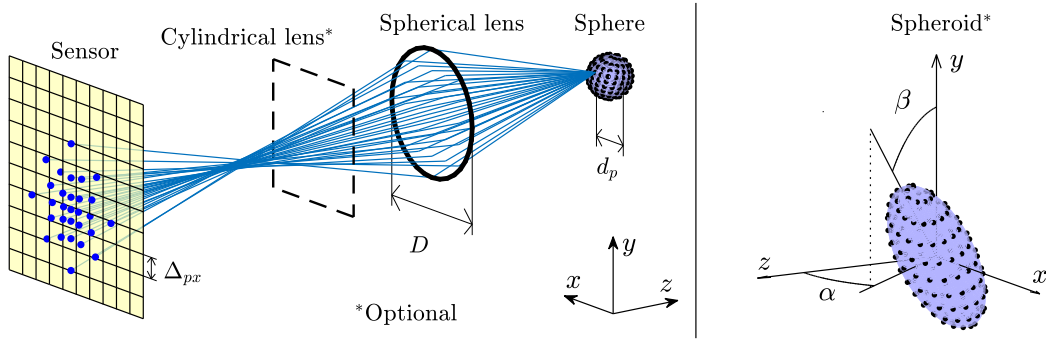
FIG. 2. General concept of MicroSIG. Tracer particles are spheres or spheroids, with light point-sources uniformly distributed on the surface. The path of each ray going through a spherical lens (and optionally also a cylindrical lens) is calculated. The intensity of one pixel is calculated as the count of rays hitting its area. A sketch of a spheroid particle with e_p = 3 and its respective orientation angles \alpha and \beta is presented on the right panel.
