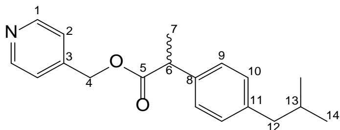
Chart 3. Structure of Py-IBU (labelling refers to carbon atoms).
