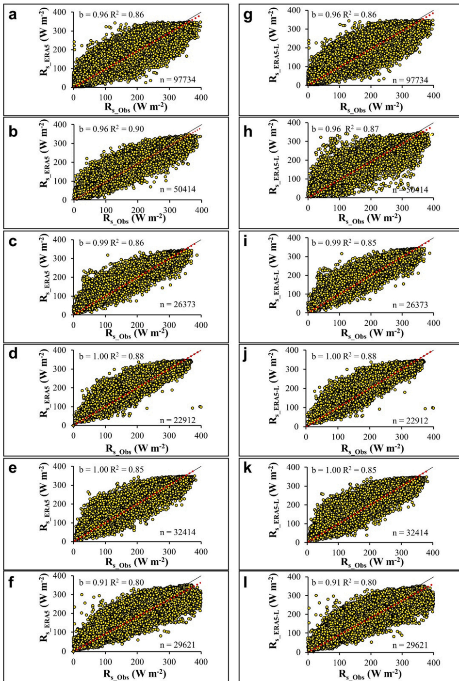
Fig. 3. Daily predicted solar radiation ( R_{s\_ERA5} and R_{s\_ERA5-L} W\ m^{-2} ) versus observed ( R_{s\_Obs} , W\ m^{-2} ) values at the irrigation districts located in Lombardy (a, g), Emilia-Romagna (b, h); Campania (c, i), Western Sicily (d, j), Eastern Sicily (e, k) and Apulia (f, l) for the period 2008–2020. The black line and red line represent the 1:1 line and linear regression line, respectively. The terms b , R^2 and n refer to the slope of the regression equation through the origin, the coefficient of determination and the number of observations, respectively.
