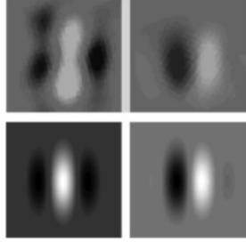
Fig. 2: First row: RFPs of two simple cells of V1 where the excitatory area is in white and the inhibitory one is in black. Second row: their approximations by Gabor functions.
