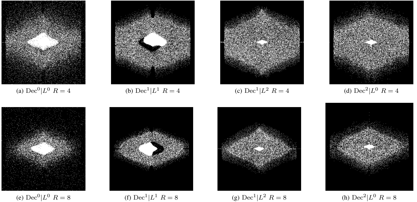
Fig. 3. undersampling masks M_\gamma \in [0, 1]^{N \times N} after training for all considered decoders (starred and non-starred versions share the same undersampling mask).
