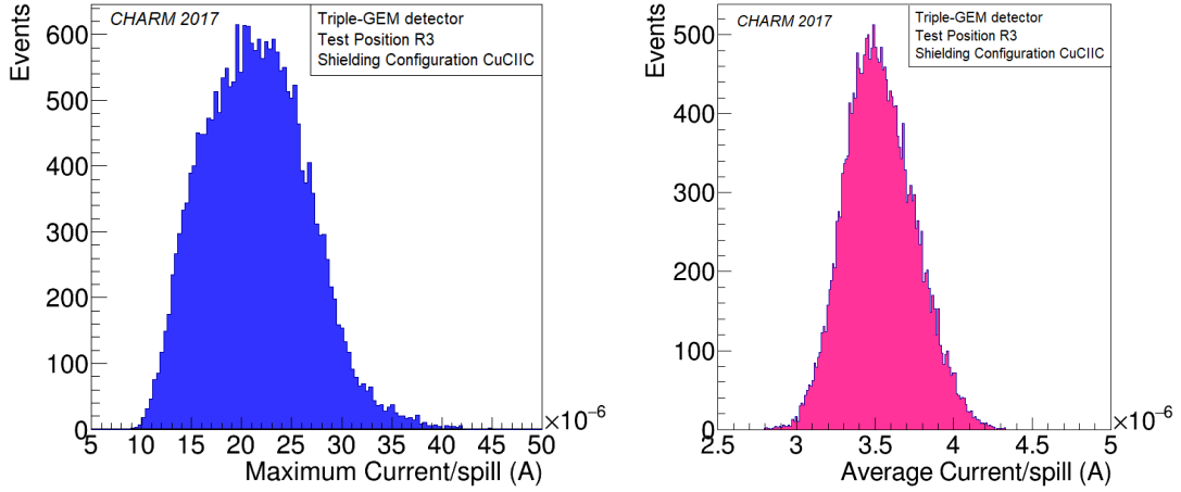
Figure 16. Maximum (left) and average (right) readout current within a spill for the Triple-GEM detector irradiated at CHARM.
