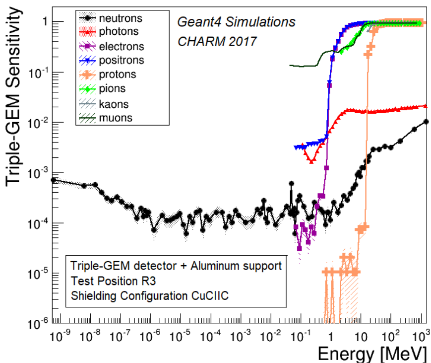
Figure 7. Sensitivity of the Triple-GEM detector exposed to the CHARM flux as a function of the energy of the incident particle for the different particle species present.
