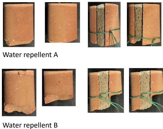
Figure 13. Penetration depth of the hydrophobic treatments observed by wetting the cylinders: a) samples treated with the product “A”; b) samples treated with the product “B”.
