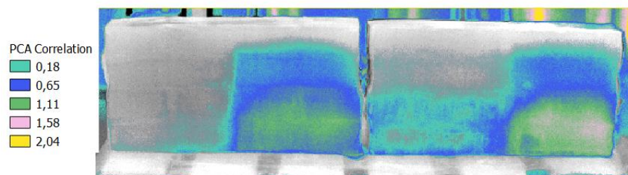
Figure 4. PCA second component: this visualisation highlights the areas where there was the most variation during the experiment.
