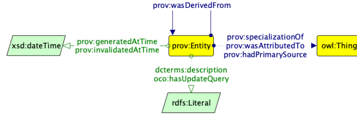
Fig. 3. The Grafoo diagram describing snapshots ( prov:Entity ) of an entity (linked via prov:specializationOf ) and the related provenance information.
