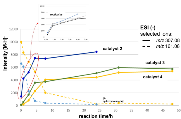
Figure 6. Intensity of ion referring to product (warfarin, m/z 307.08) vs reaction time. Dotted lines refer to the intensity of 4-hydroxycoumarin ( m/z 161.08). Lines stopped at 24 h refer to the reactions catalyzed by diamine-cyclohexane. All data are reported without any correction.
