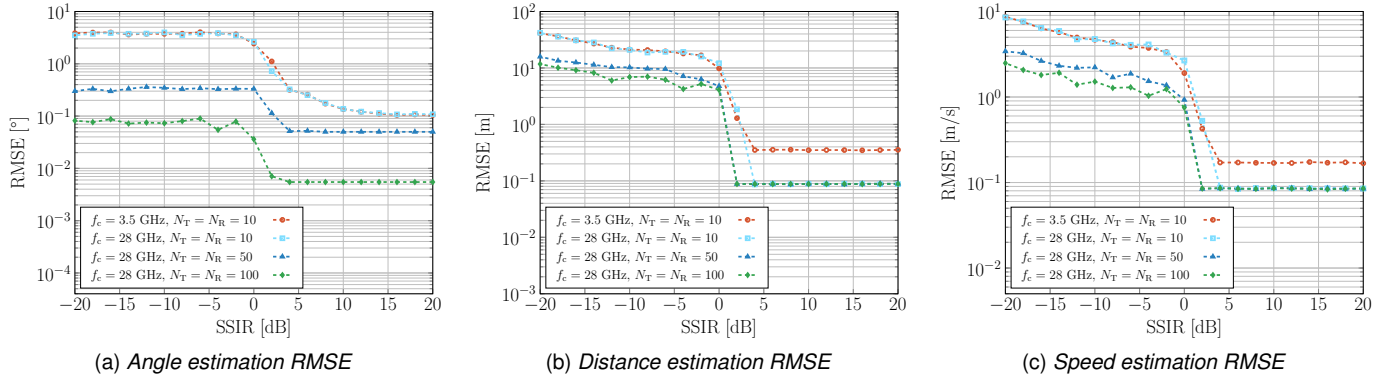
Fig. 2. Sensing performance as a function of the SSIR for DoA, distance, and speed estimates, when \text{SNR} = -20 dB.
