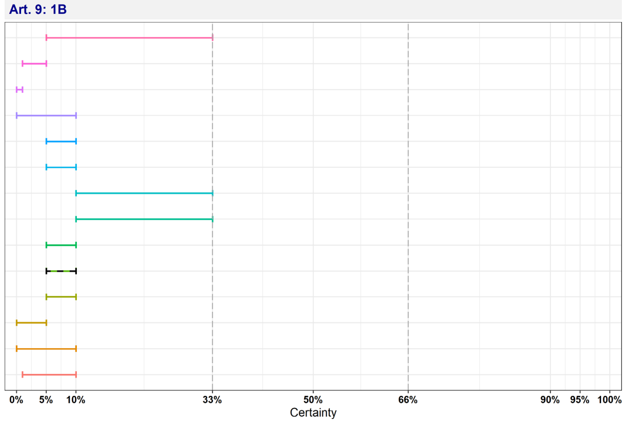
Figure A.9: Individual probability ranges reflecting non-fulfilment of criterion 1B (the disease is present in the whole or part of the Union territory with an endemic character and (at the same time) several Member States or zones of the Union are free of the disease) after the collective judgement
