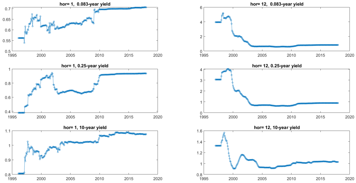
Figure 4: Recursive relative RMSFE of the JSZ-VAR-CSV versus the random walk. Recursive means are computed starting from January 1996.
