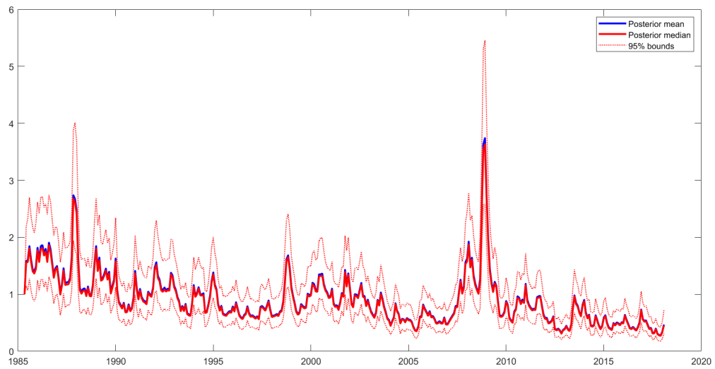
Figure 2: Posterior distribution of the common stochastic volatility process \lambda_t
