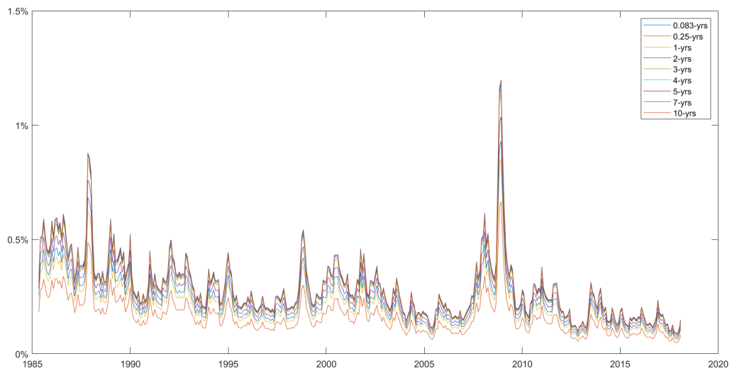
Figure 3: Volatilities for each yield (posterior medians)
