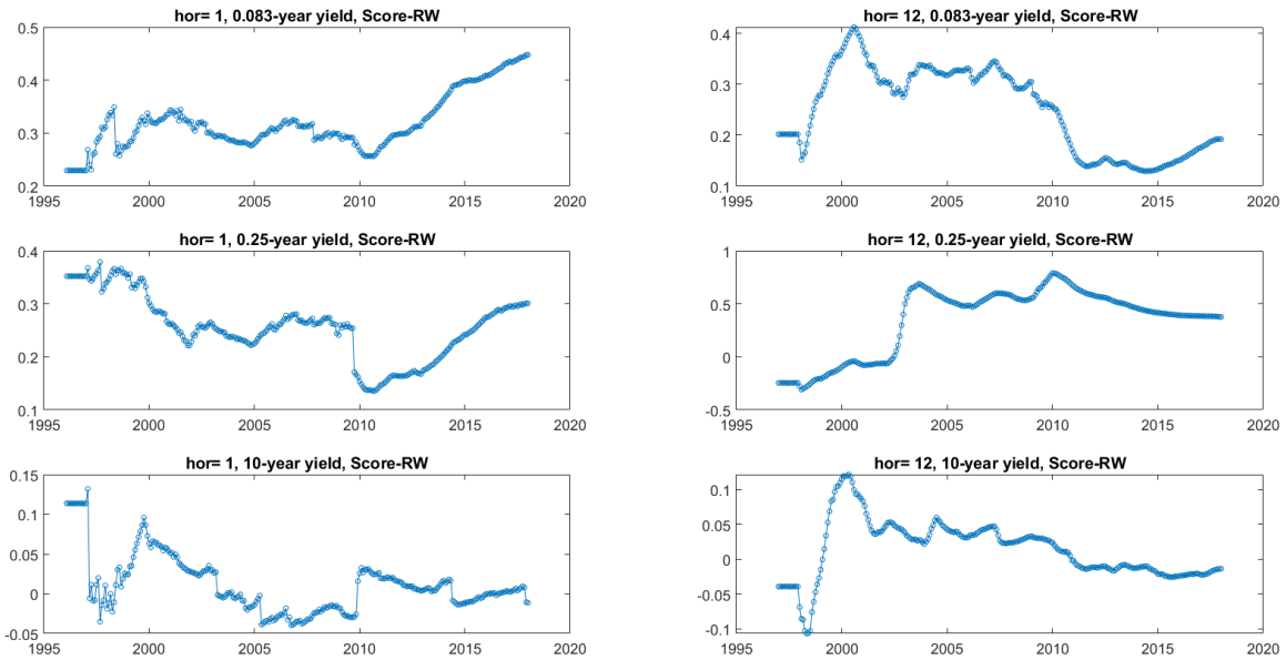
Figure 5: Recursive difference in SCORE of the JSZ-VAR-CSV versus the random walk. Recursive differences are computed starting from January 1996.
