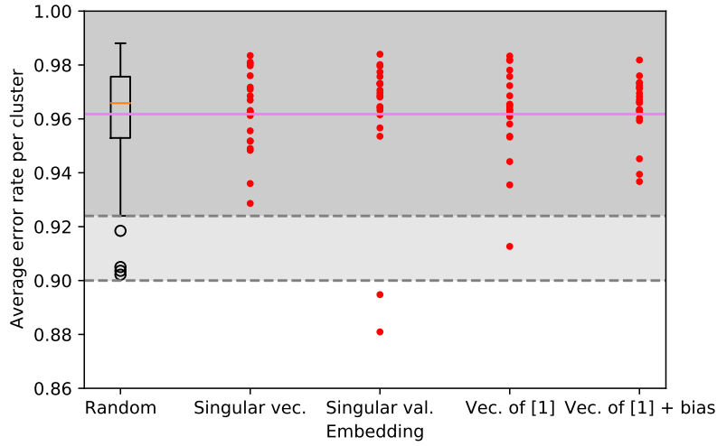
Fig. 4: Average error rate per cluster. Representation of nodes with a vector of singular values identifies two clusters with significantly higher anomaly rate than the whole population.
