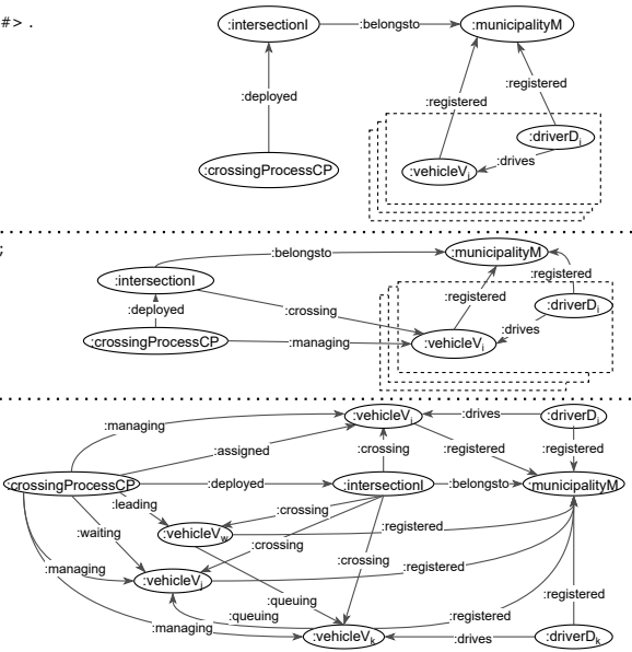
Fig. 15. Evolution of the knowledge graph in the mobility intelligence scenario.
