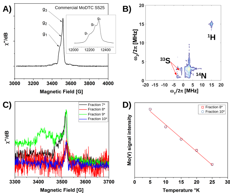
Figure 4. EPR spectra of the MoDTC samples. (A) Echo field sweep EPR spectrum of the commercial S525 mixture measured at the X-band and at 20 K, with the Q-band echo spectrum at 20 K as an inset. (B) 2D-HYSCORE spectrum at 20 K of the commercial S525 mixture. (C) Echo field sweep EPR spectrum of the separated fractions measured at the X-band and at 5 K. (D) Intensity of the Mo(V) signal vs the temperature, indicating the Curie behavior and, therefore, the paramagnetic nature of the species in fractions 8* and 10*.
