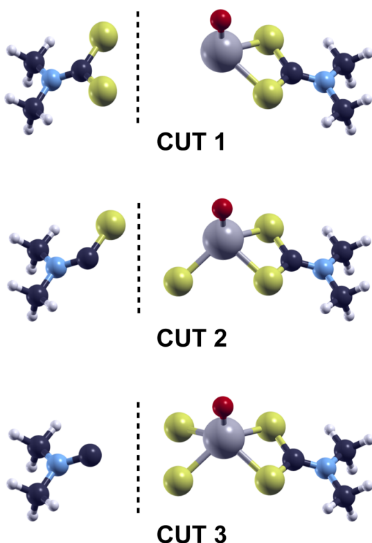
Figure 7. Schematic representation of the dissociation patterns of mMoDTC.
