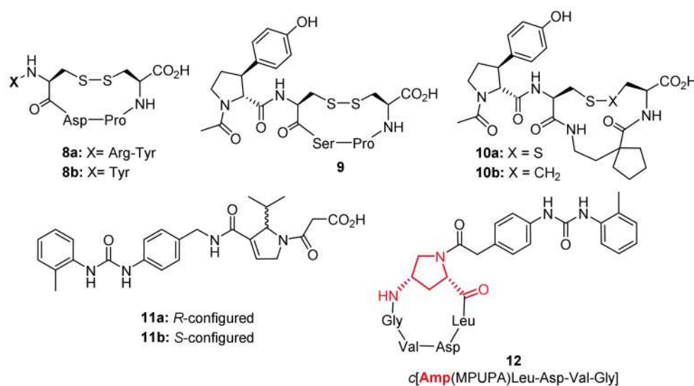
Figure 4. Known cyclic peptides ( 8a , 8b , and 9 ), their spirocyclic analogues ( 10a , 10b ), the dehydro- \beta -proline peptidomimetics 11a and 11b , and the novel Amp-based cyclopentapeptidomimetic 12 used for docking studies in this work.
