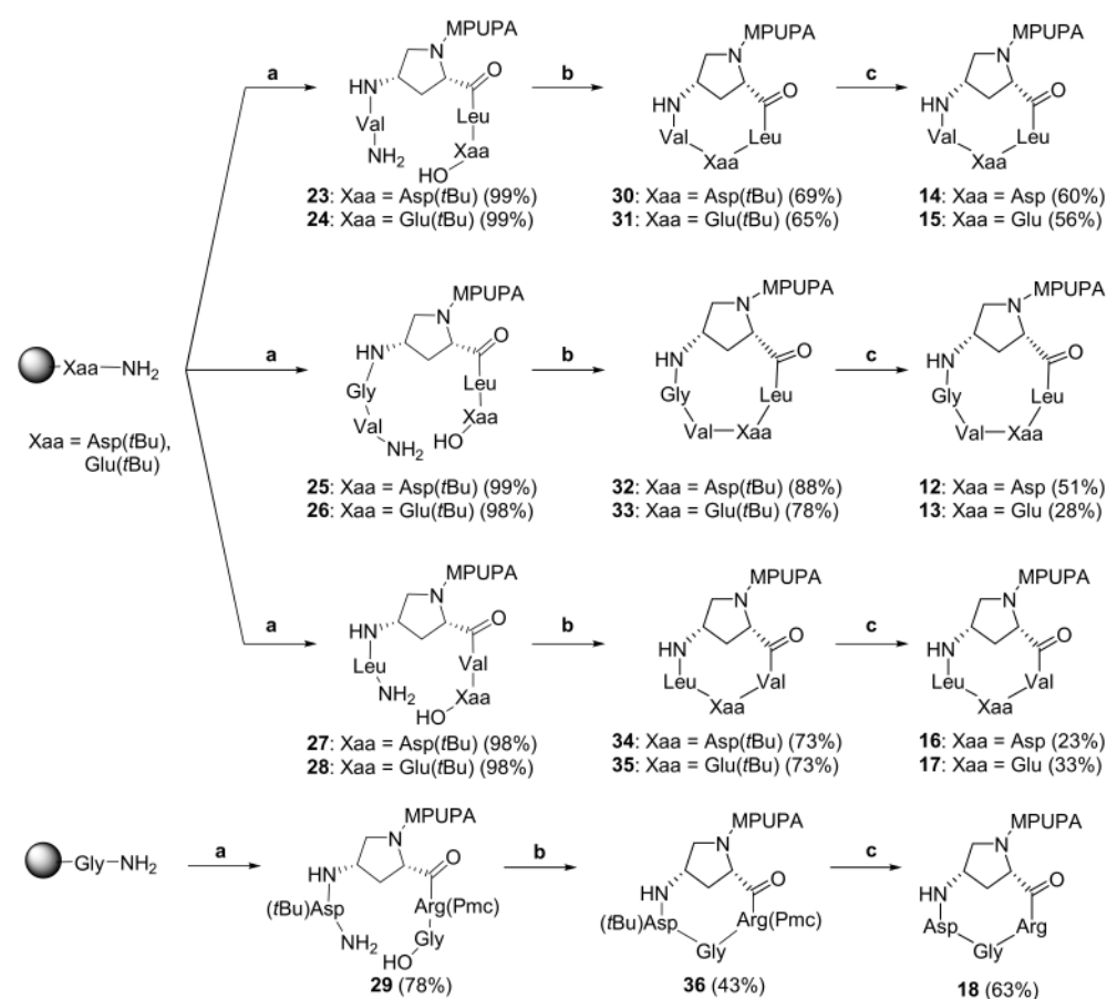
Scheme 2. Synthesis of Amp(MPUPA)-based target compounds 12–18 . Reagents and conditions: (a) Fmoc-SPPS strategy. Coupling: Fmoc-amino acid, HATU, HOAt, collidine, DMF, rt. Fmoc cleavage: 20% piperidine in DMF, rt. Sequence of addition to obtain compounds: ( 23 , 24 ) Fmoc-Leu-OH, Fmoc-Amp(MPUPA)-OH ( 22 ), Fmoc-Val-OH; ( 25 , 26 ) Fmoc-Leu-OH, Fmoc-Amp(MPUPA)-OH ( 22 ), Fmoc-Gly-OH, Fmoc-Val-OH; ( 27 , 28 ) Fmoc-Val-OH, Fmoc-Amp(MPUPA)-OH ( 22 ), Fmoc-Leu-OH; ( 29 ) Fmoc-Arg(Pmc)-OH, Fmoc-Amp(MPUPA)-OH ( 22 ), Fmoc-Asp( t Bu)-OH. Resin cleavage: AcOH/TFE/DCM (1:1:3), rt. (b) Cyclization: HATU, HOAt, collidine, DCM/DMF (15:1), 1–3 mM, rt. (c) Deprotection: TFA/TIS/H 2 O (95:2.5:2.5), rt.
