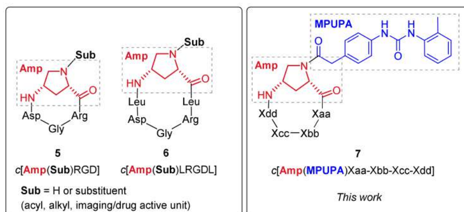
Figure 2. Amp-based cyclopeptides directed to RGD-recognizing \alpha_V\beta_3 , \alpha_V\beta_5 , and \alpha_V\beta_6 integrins (compounds 5 and 6 ) [30–40], and general structure of cyclopeptidomimetics 7 designed and synthesized to target \alpha_4\beta_1 integrin in the present study.
