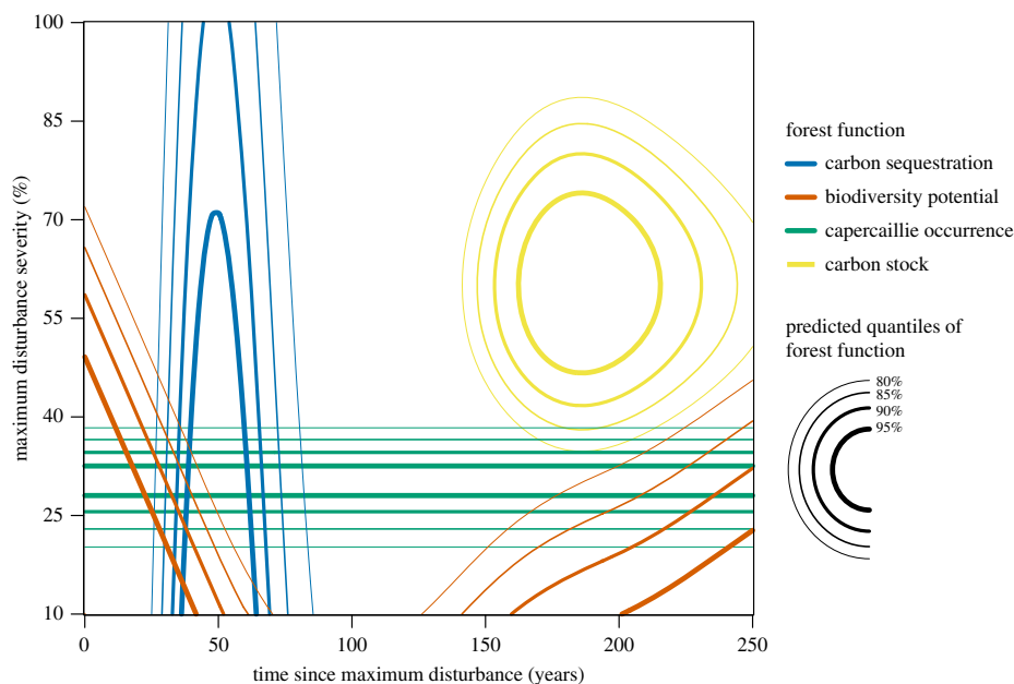
Figure 2. Maxima of forest functions along the gradients of maximum disturbance severity and time since that event. Isolines represent upper percentiles (greater than 80%) of GAMM-predicted values of the forest functions.
