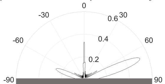
Fig. 7. Radiation pattern of the lossless anomalous reflector in [20]. Setup: normal incidence and the desired angle of reflection is 70 degrees.
