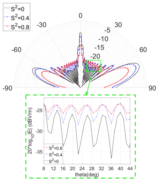
Fig. 8. Far-field (dBV/m) scattering pattern of the lossless anomalous reflector considered in [20] in the absence of diffuse scattering (reference black curve), and in the presence of 40% (blue curve) and 80% (red curve) of the incident power diverted into diffuse scattering.
