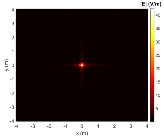
Fig. 6. Reradiated field [V/m] from a 7 \times 7 \text{ m}^2 focusing lens. Except for the phase profile of the metasurface, the setup is the same as for Fig. 4.
