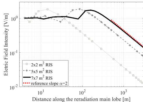
Fig. 11. Local average of the amplitude of the radiated electric field by an ideal phase-gradient reflector with E_i = 1 V/m, \theta_i = 0^\circ , \theta_r = 30^\circ . The curves are computed by using (16) as a function of the distance and for different sizes of the RIS at the frequency f = 3 GHz.
