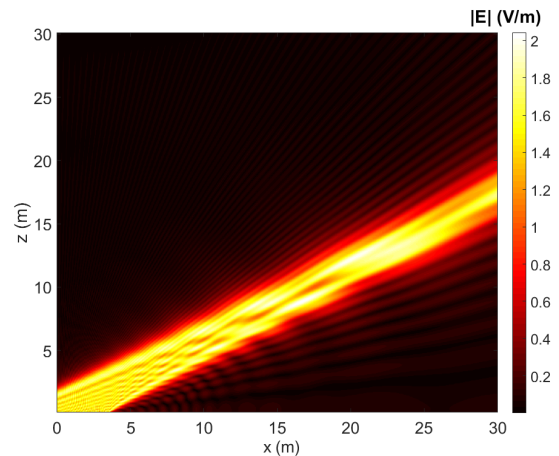
Fig. 4. Reradiated field [V/m] in the xz plane from a 7 \times 7 m 2 RIS that is located in the xy plane and is centered at the origin. Setup: 3 GHz operating frequency, normal incidence, reflection towards the angle of 60 degrees.
