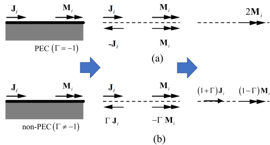
Fig. A1. Conventional (a) and modified (b) method of image currents. The image currents replace the presence of the object (scatterer, i.e., the RIS) for the purpose of calculating the field outside of it.
