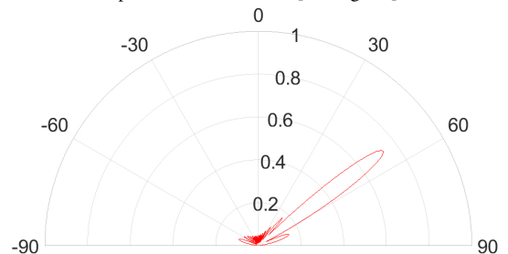
Fig. 10. Far-field radiation pattern ( \rho = 0, S = 0, m = 0.9 ) corresponding to the lossy phase-gradient metasurface reported in [33, Fig 2.e]. The corresponding benchmark radiation pattern is available in [33, Fig 2.f].
