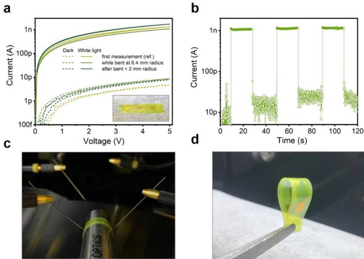
Figure 6. Demonstration of working device on flexible substrate. a, I-V characteristics in dark conditions and under white light illumination ( \sim 110 \text{ mW/cm}^2 ) of a NCs film on polyethylene naphthalate (PEN) substrate (inset) contacted with thermal evaporated Ag contacts, with a channel length of 100 \mu\text{m} . b, Photocurrent generated by switching the same white light ON and OFF over time, demonstrating measurement reproducibility. c. Photograph of the device working under bending conditions. d, Photograph of the bent test with \sim 2 \text{ mm} bending radius.
