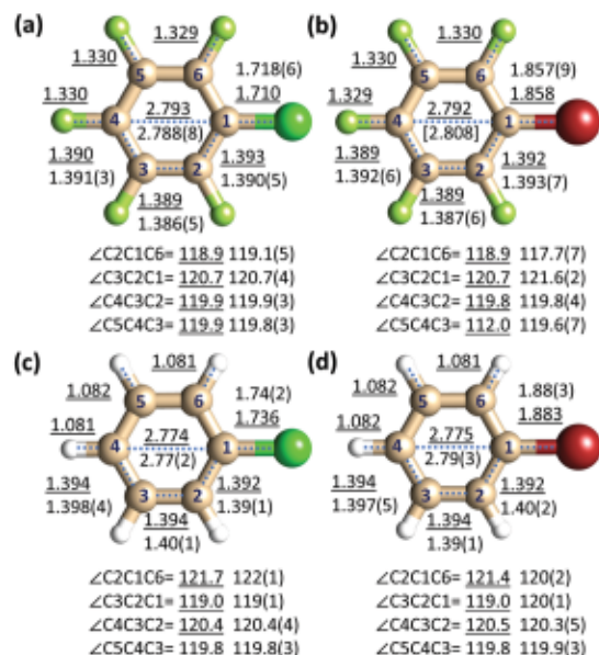
Fig. 4 Geometries of (a) C_6F_5Cl , (b) C_6F_5Br , (c) C_6H_5Cl and (d) C_6H_5Br . MP2/aug-cc-pVTZ parameters (underlined values) and experimental values (normal font). Distances in Å, angles in degrees. The R(C1C4) parameter in C_6F_5Br (in square brackets) is fixed to 2.808 Å (see text for details). Error in parentheses in units of the last digit. Rotational constants of C_6H_5Cl and C_6H_5Br taken from ref. 33 and 34 respectively.
