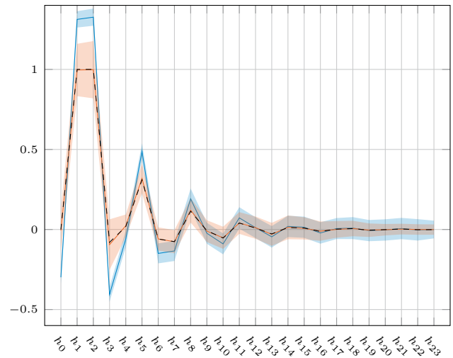
Fig. 4. True truncated impulse response of the IIR system (53) (dashed black), mean of its estimate obtained with Algorithm 1 in red and with Algorithm (Diversi et al., 2008) in blue and associated standard deviations in transparency. Monte Carlo simulation of 1000 runs performed with N = 10000 and \text{SNR} = 5\text{dB} .
